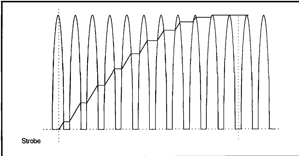
FIGURE 6: Servo Burst Acquisition ( SG = \overline{RESET} = 1 )
