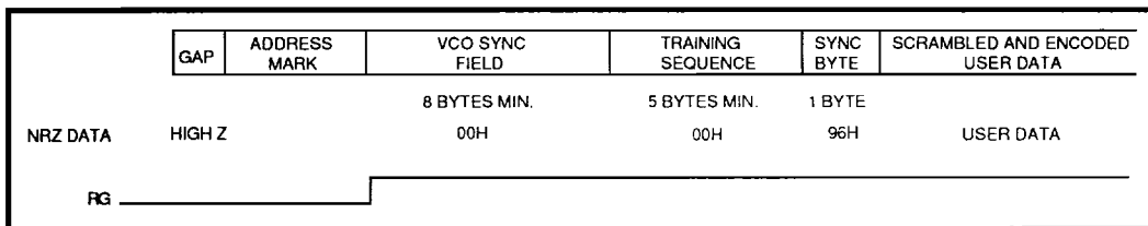
FIGURE 10: Sector Read Sequence
