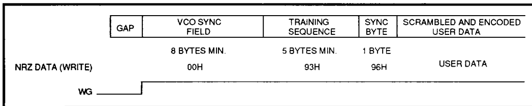
FIGURE 9: Sector Write Sequence
