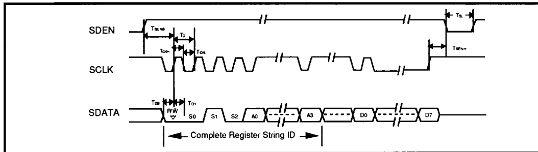
FIGURE 8: Serial Interface Timing
