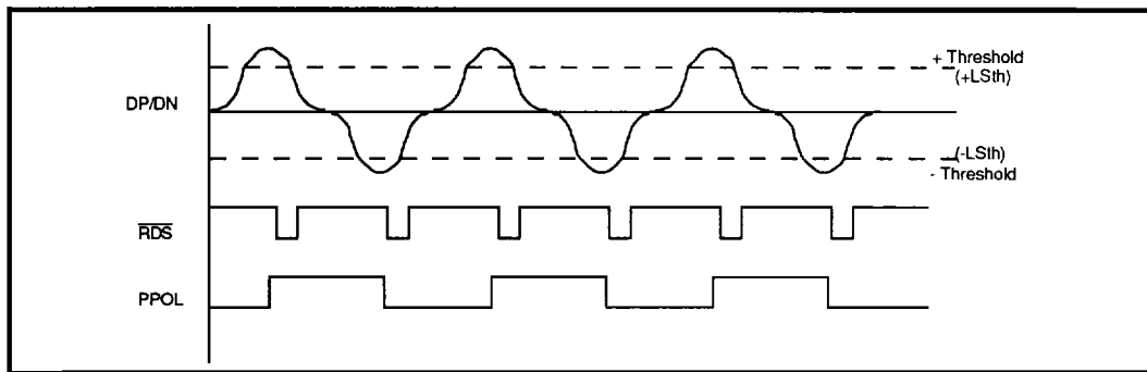
FIGURE 7: \overline{RDS} and PPOL vs. DP/DN Relationship
