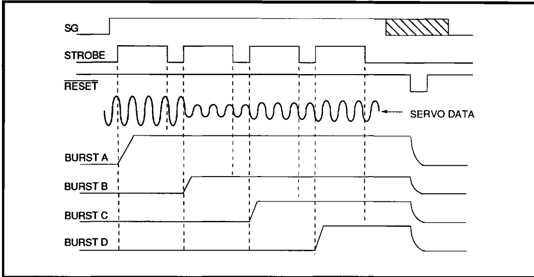
FIGURE 5: Servo Capture Timing Diagram
