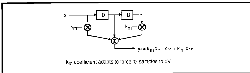
FIGURE 2: Block Diagram of 3-Tap Adaptive Equalizer
