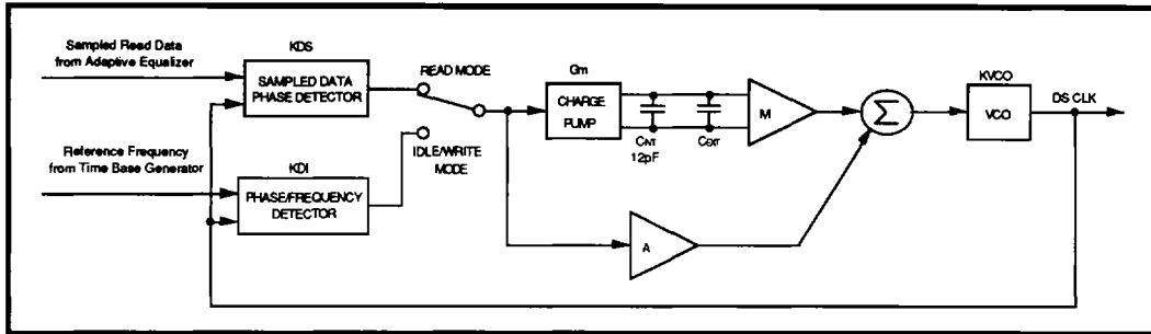
FIGURE 3: Data Synchronizer Phase Locked Loop
