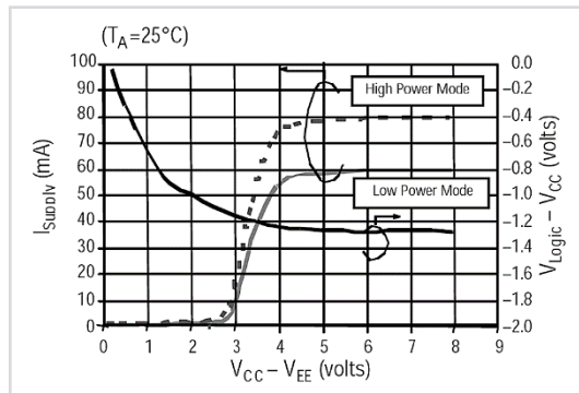
Figure 5. Typical supply current & V_{Loic} vs. supply voltage
