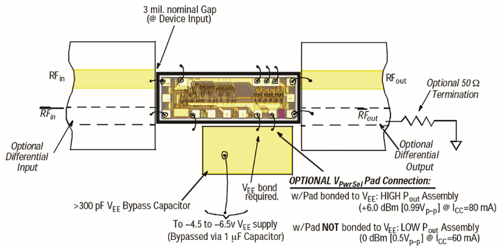
Figure 3. Assembly diagrams
