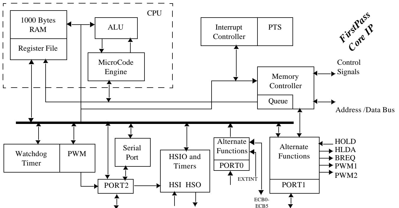
Figure 1. UT80C196KD Microcontroller
