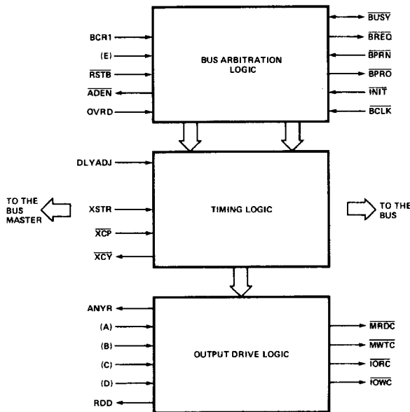
Figure 1. Block Diagram
