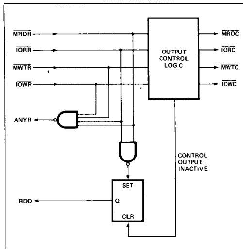
Figure 4a. 8218 Control Logic
