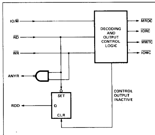
Figure 4b. 8219 Control Logic
