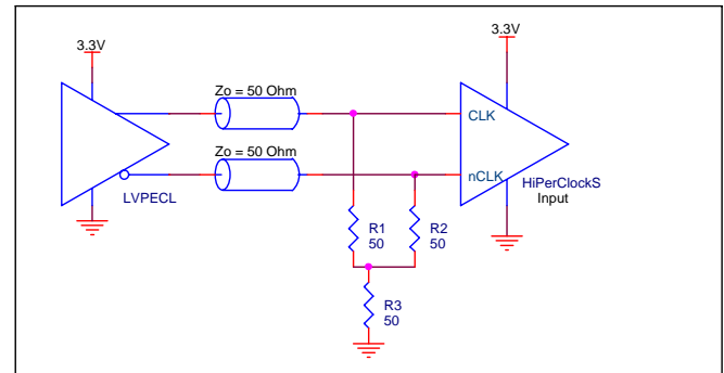
FIGURE 1B. CLK/nCLK INPUT DRIVEN BY 3.3V LVPECL DRIVER
