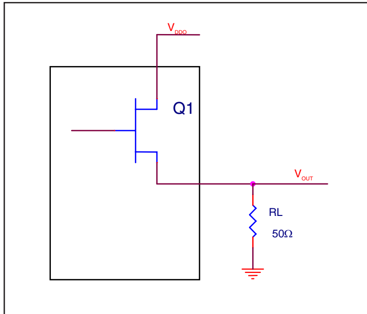
FIGURE 2. LVHSTL DRIVER CIRCUIT AND TERMINATION
