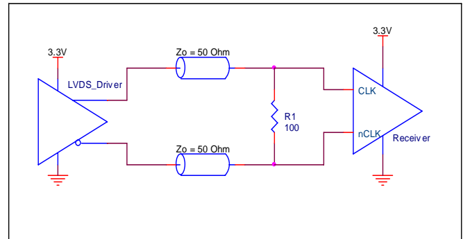
FIGURE 1D. CLK/nCLK INPUT DRIVEN BY 3.3V LVDS DRIVER
