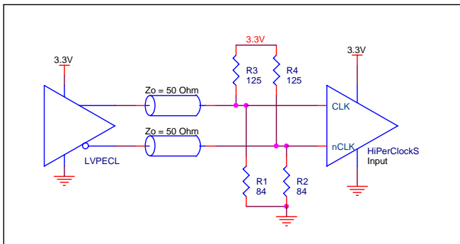
FIGURE 1C. CLK/nCLK INPUT DRIVEN BY 3.3V LVPECL DRIVER
