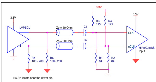
FIGURE 1E. CLK/nCLK INPUT DRIVEN BY 3.3V LVPECL DRIVER WITH AC COUPLE
