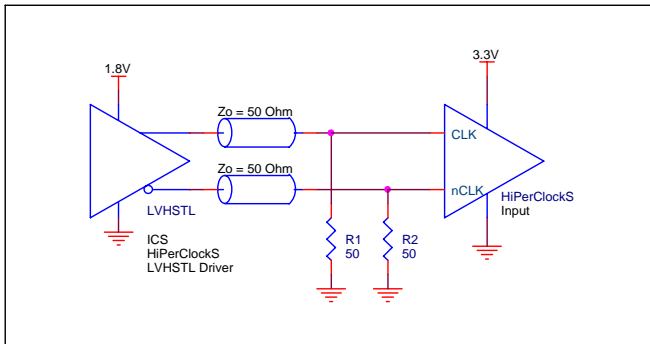
FIGURE 1A. CLK/nCLK INPUT DRIVEN BY LVHSTL DRIVER
