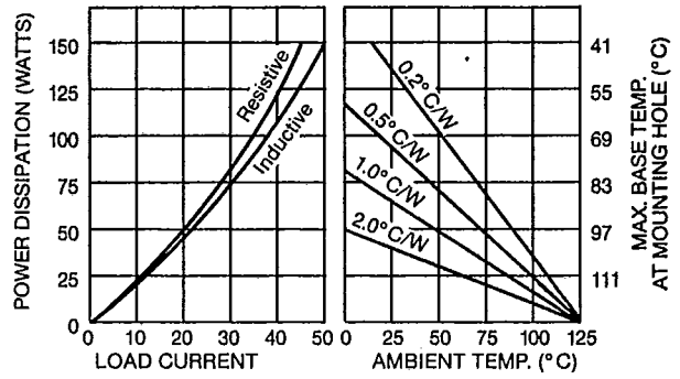
FIGURE 2 — THERMAL DERATING CURVES, M2540 CIRCUITS 1,2,3 & 6
