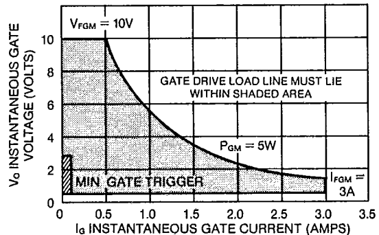
FIGURE 7 — GATE CHARACTERISTICS
