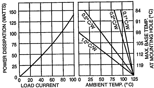
FIGURE 1 — THERMAL DERATING CURVES, M5050 CIRCUITS 4,5,7 & 8
