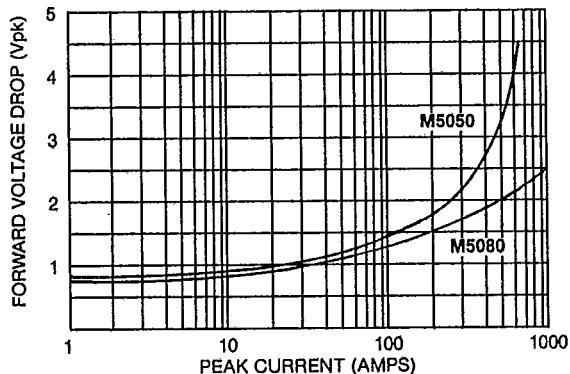
FIGURE 5 — FORWARD VOLTAGE DROP VS. PEAK CURRENT (@ 125°C)
