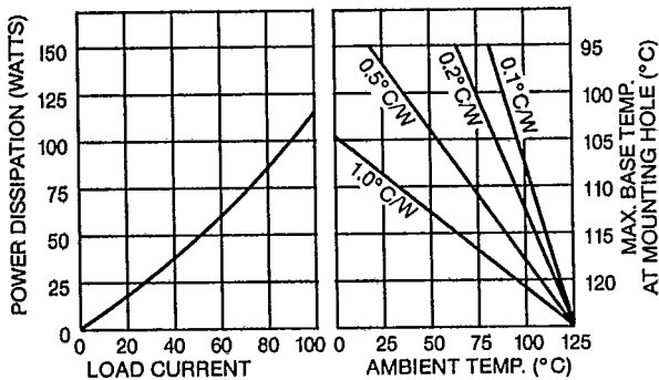
FIGURE 3 — THERMAL DERATING CURVES, M5080 CIRCUITS 4,5,7 & 8
