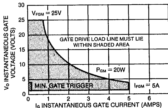
FIGURE 7 — GATE CHARACTERISTICS
