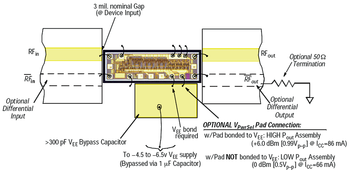
Figure 3. Assembly diagrams
