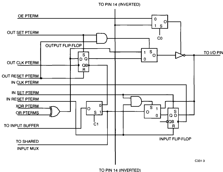
Figure 1. I/O Macrocell
