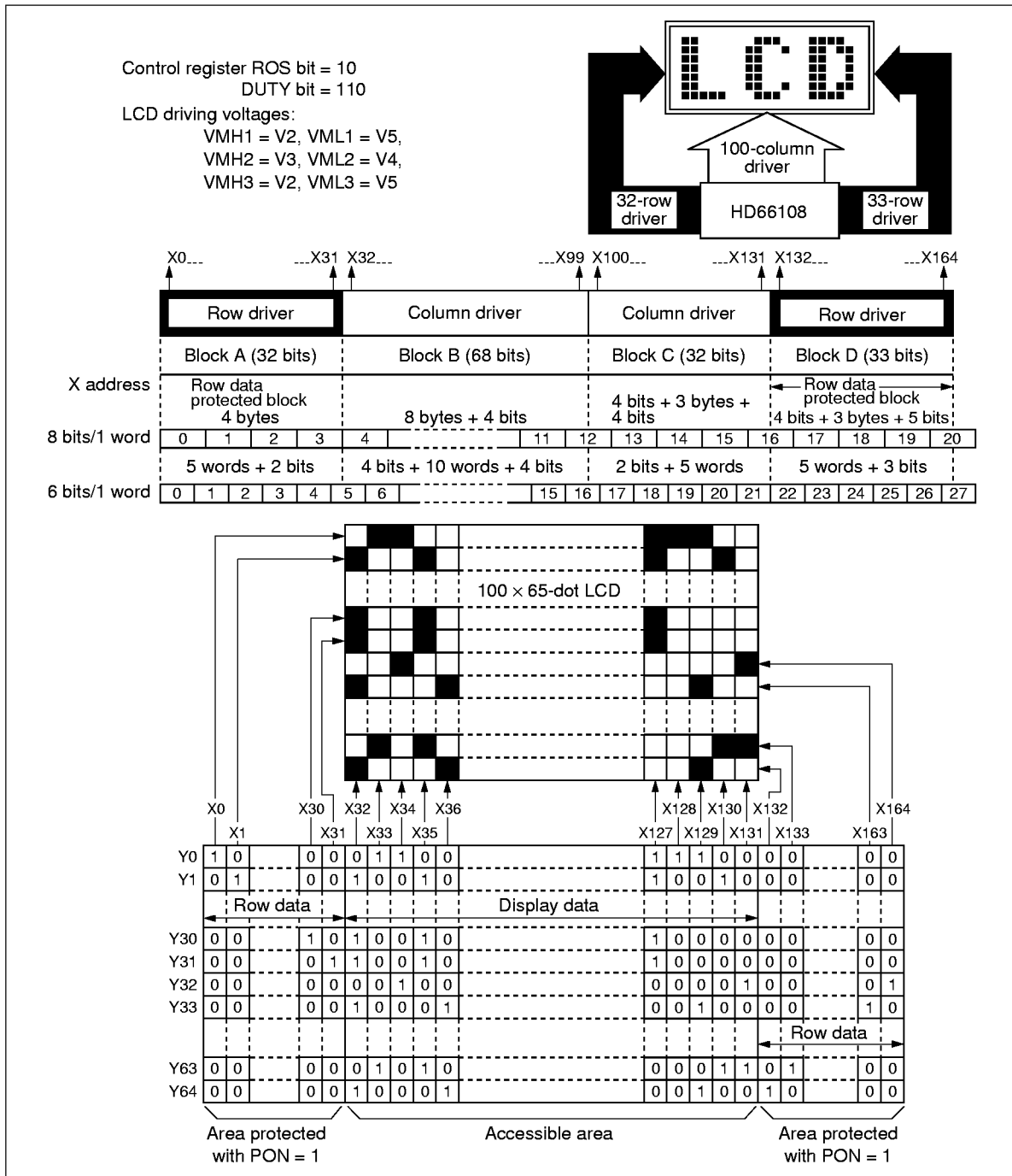
Figure 17 Relationship between Row Data and Display (65-Row Output from the Left and Right Sides, 1/66 Multiplexing Duty Ratio)
