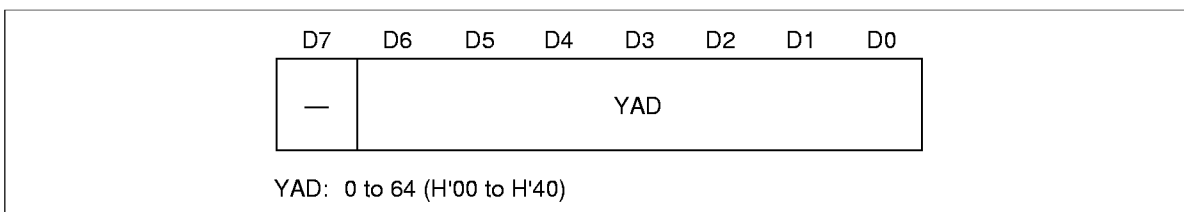
Figure 30 Y Address Register
