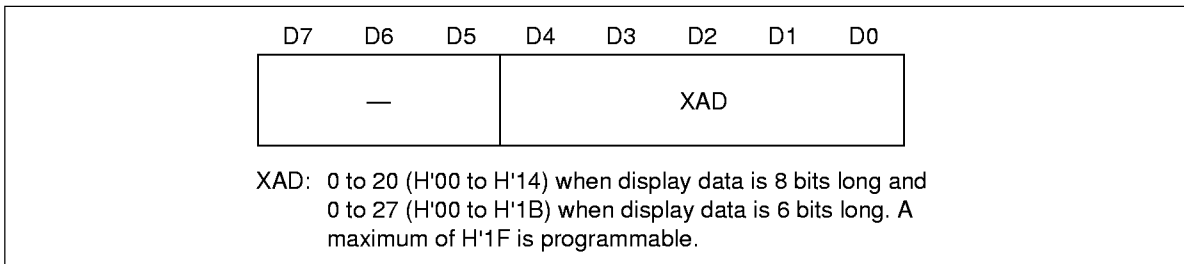
Figure 29 X Address Register
