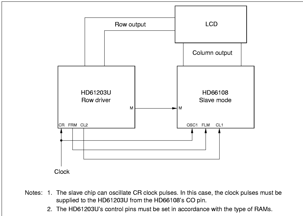
Figure 26 Configuration Using One HD66108 Chip with Another Row Driver (HD61203U)
