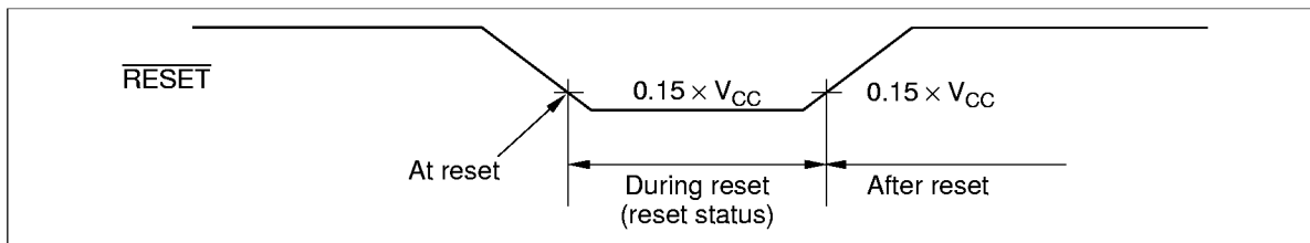
Figure 34 Reset Definition
