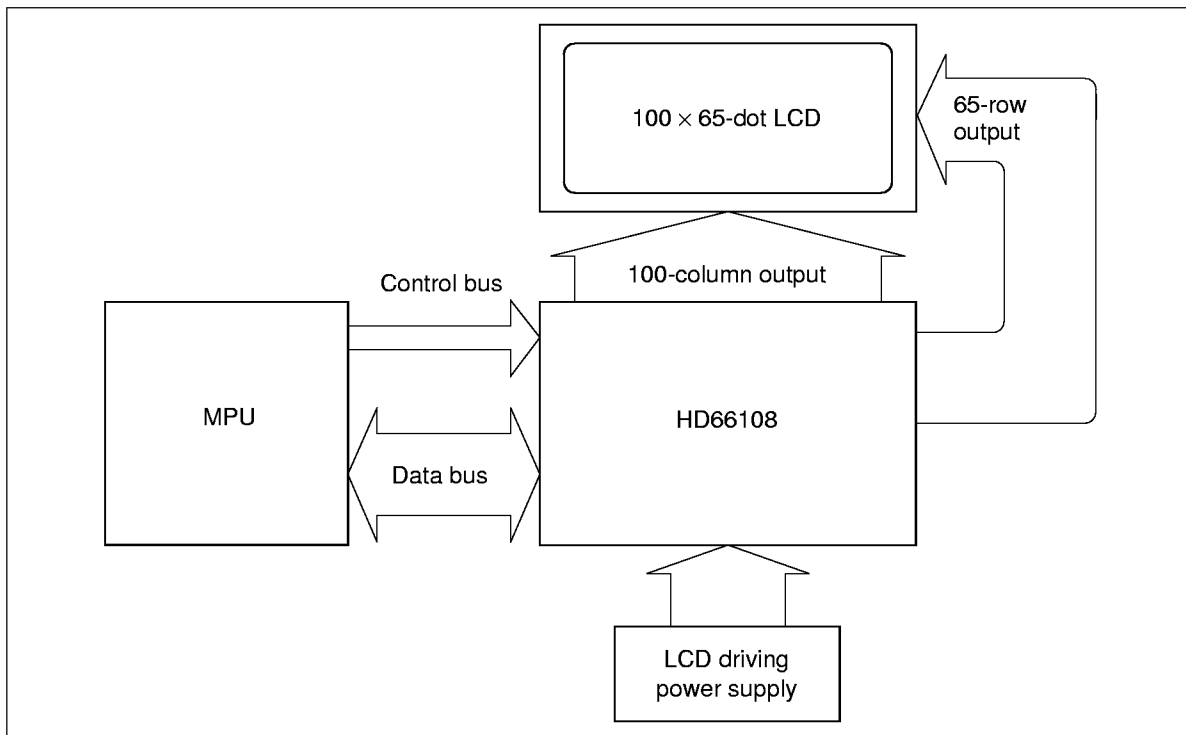
Figure 1 Basic System Configuration (1)
