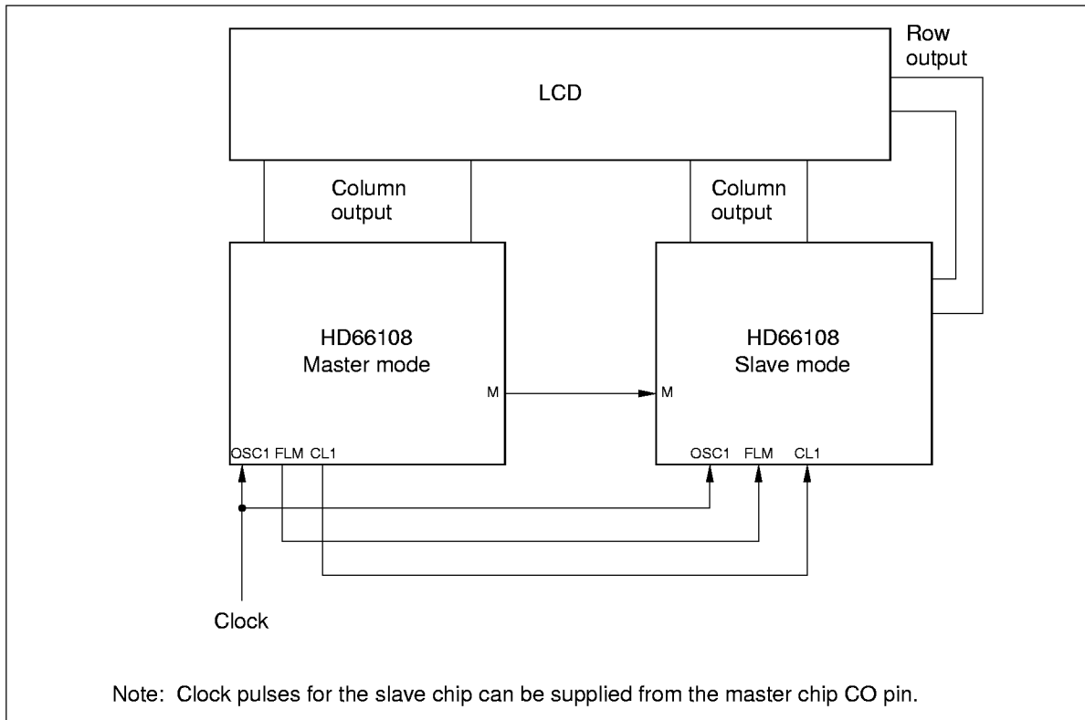
Figure 25 Configuration Using Two HD66108 Chips (2)
