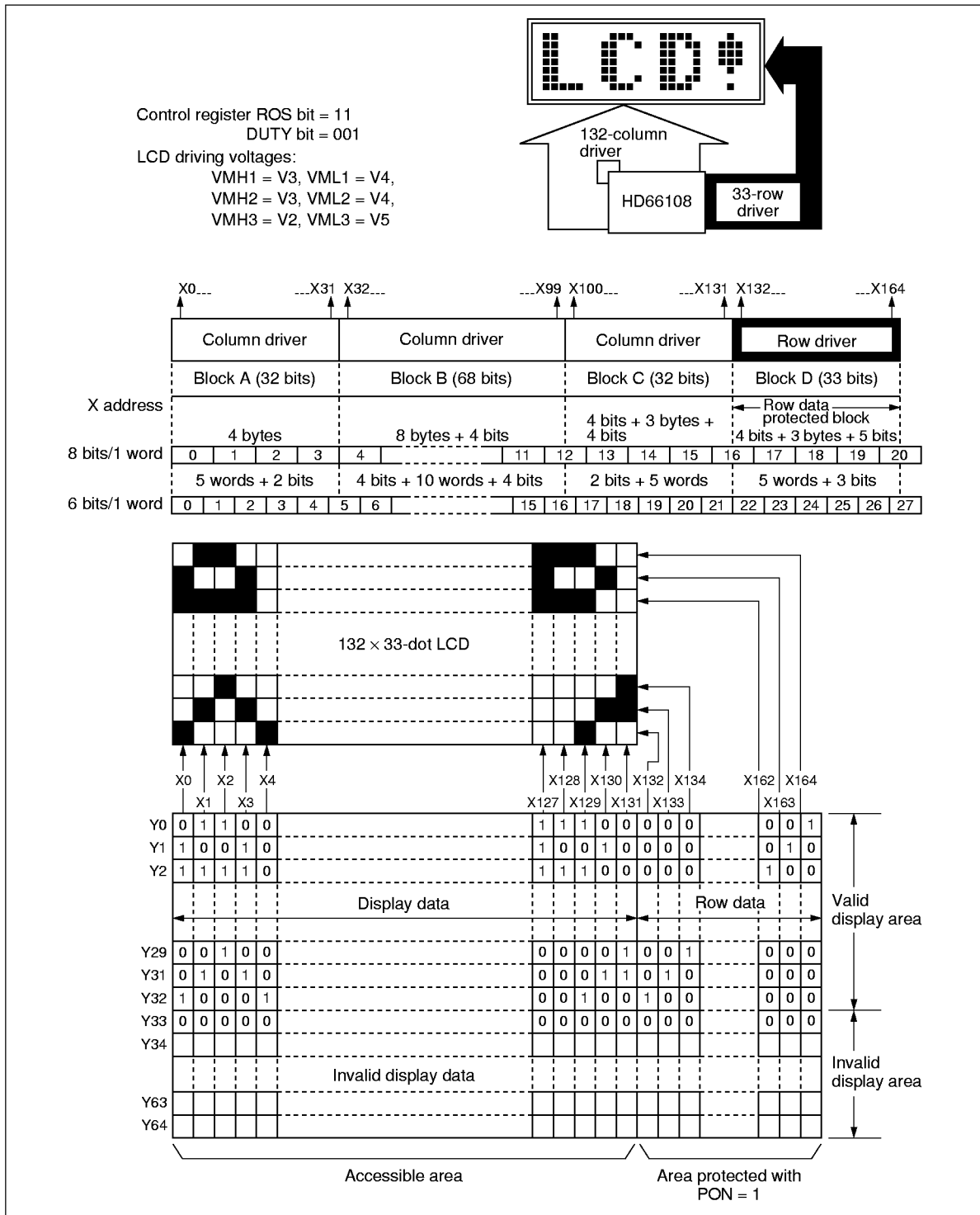
Figure 18 Relationship between Row Data and Display (33-Row Output from the Right Side, 1/34 Multiplexing Duty Ratio)
