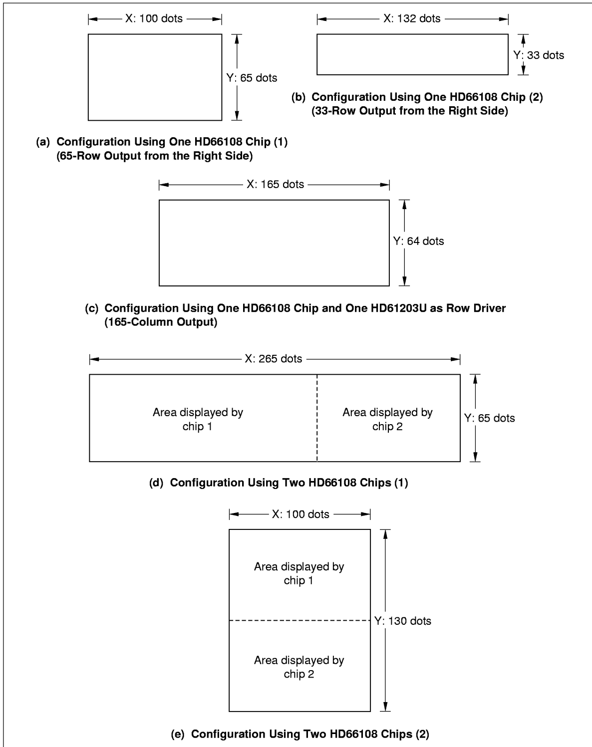
Figure 3 Relationship between System Configurations and Display Sizes
