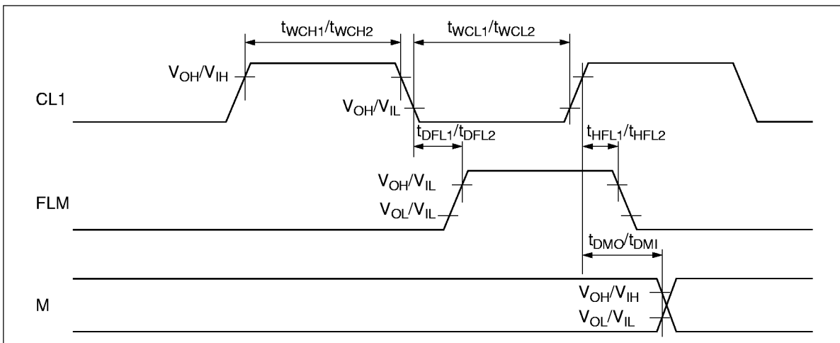
Figure 38 LCD Interface Timing
