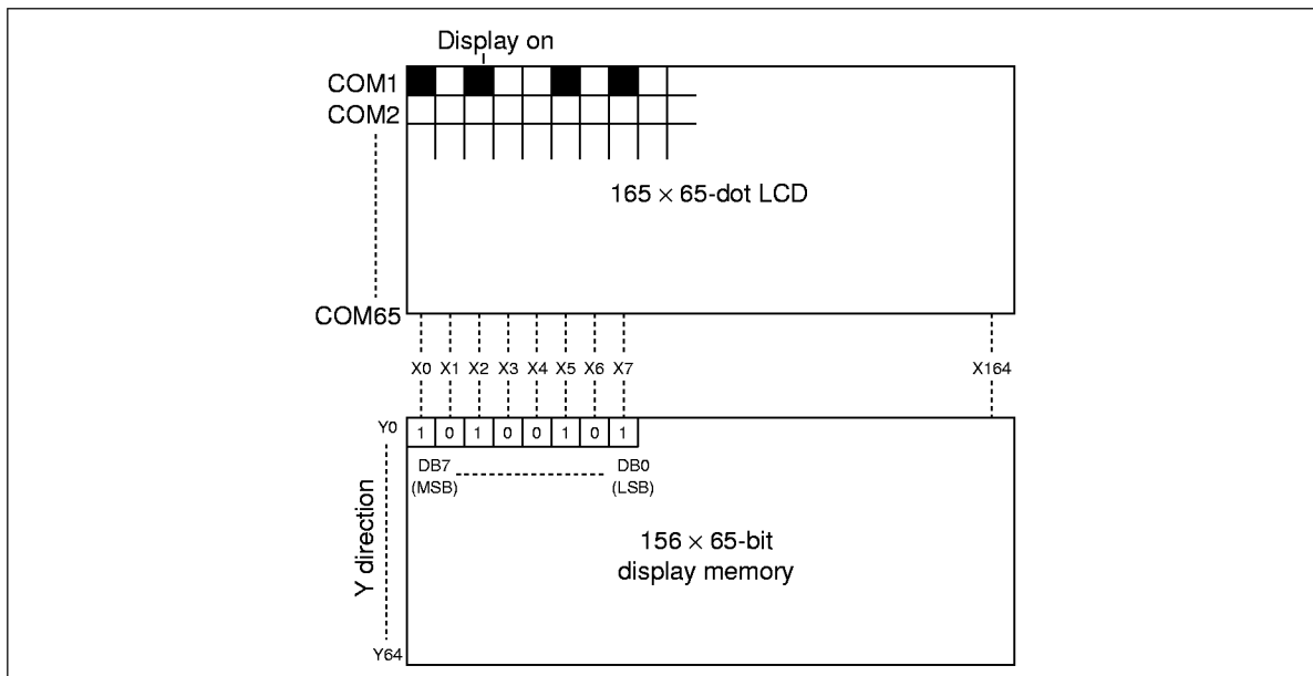
Figure 4 Relationship between Memory Construction and Display
