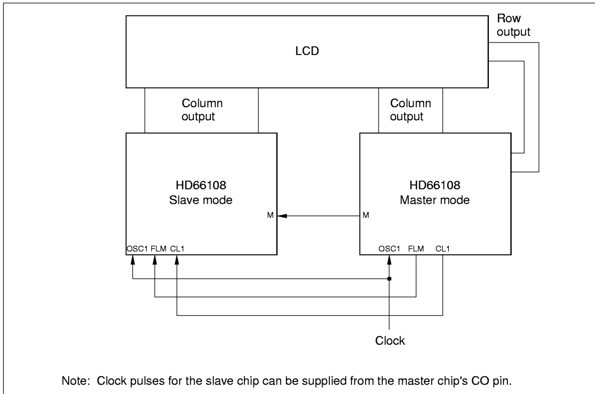
Figure 24 Configuration Using Two HD66108 Chips (1)
