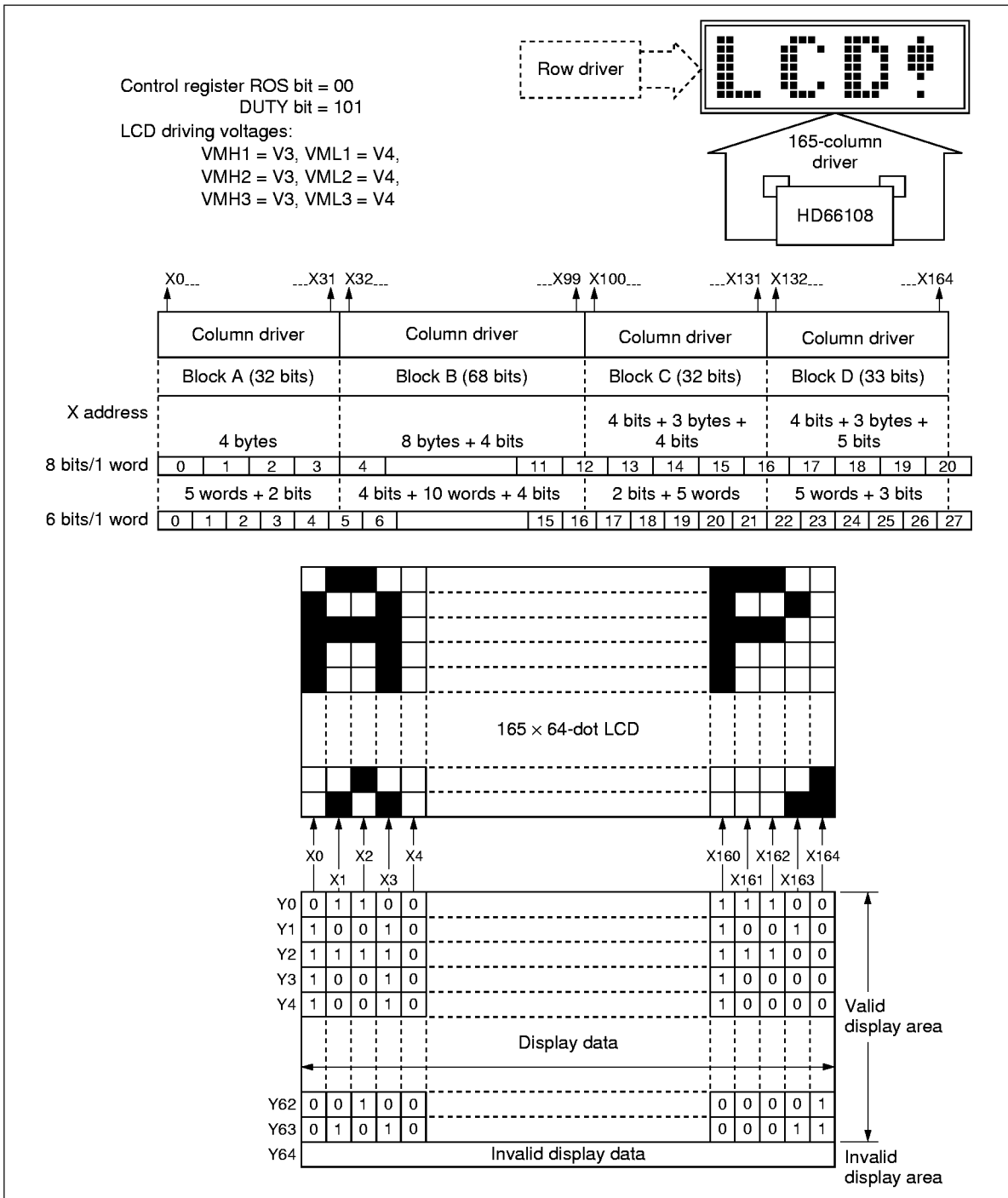
Figure 15 Relationship between Row Data and Display (165-Column Output, 1/64 Multiplexing Duty Ratio)
