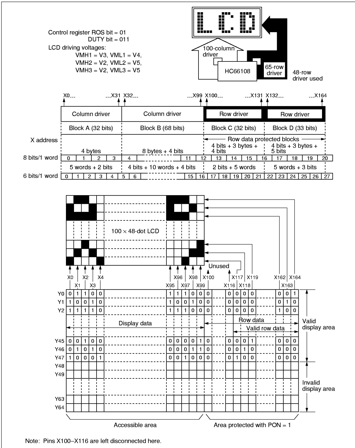
Figure 19 Relationship between Row Data and Display (65-Row Output from the Right Side, 1/48 Multiplexing Duty Ratio)
