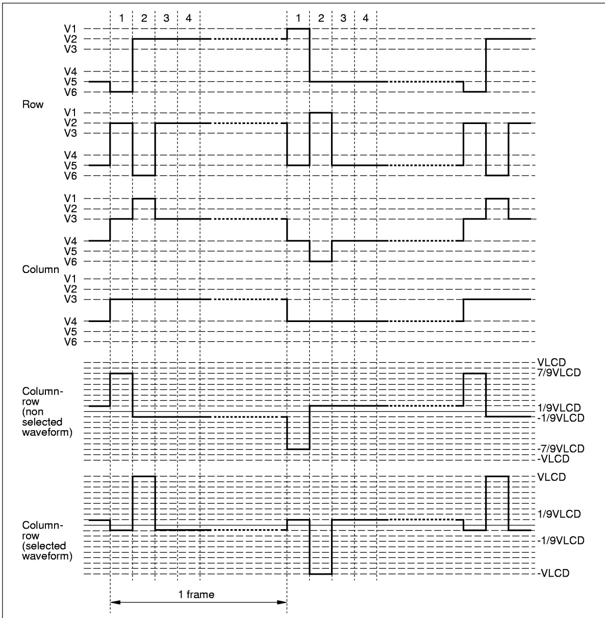
Figure 20 LCD Driving Voltage Waveforms
