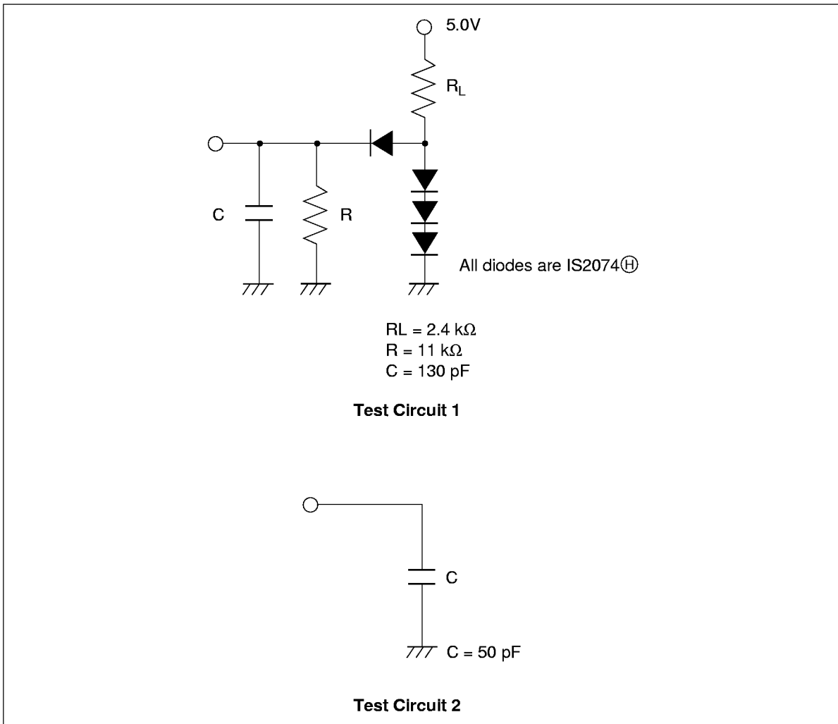
Figure 39 Load Circuits
