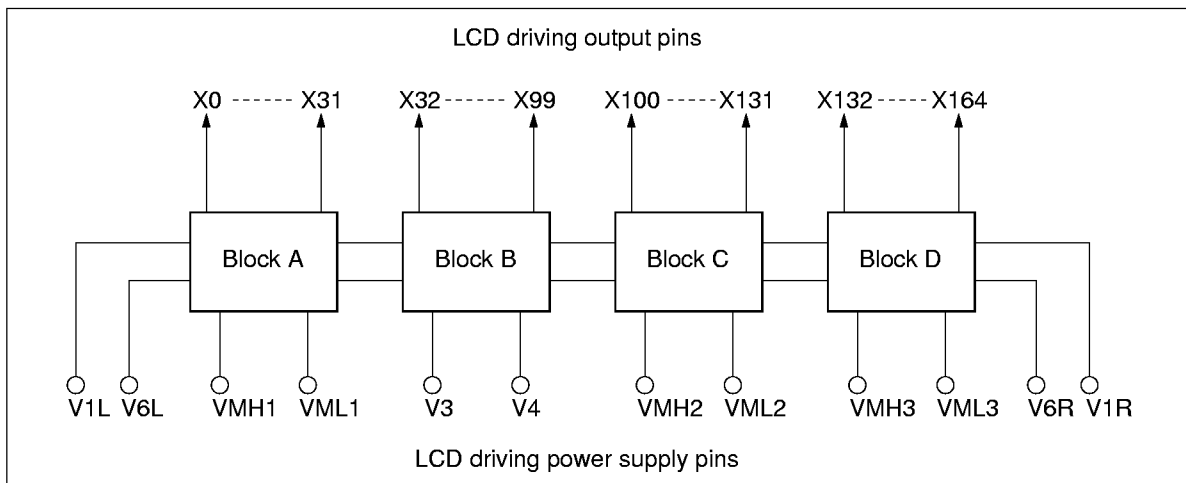
Figure 21 Relationship between Blocks and LCD Driving Voltages
