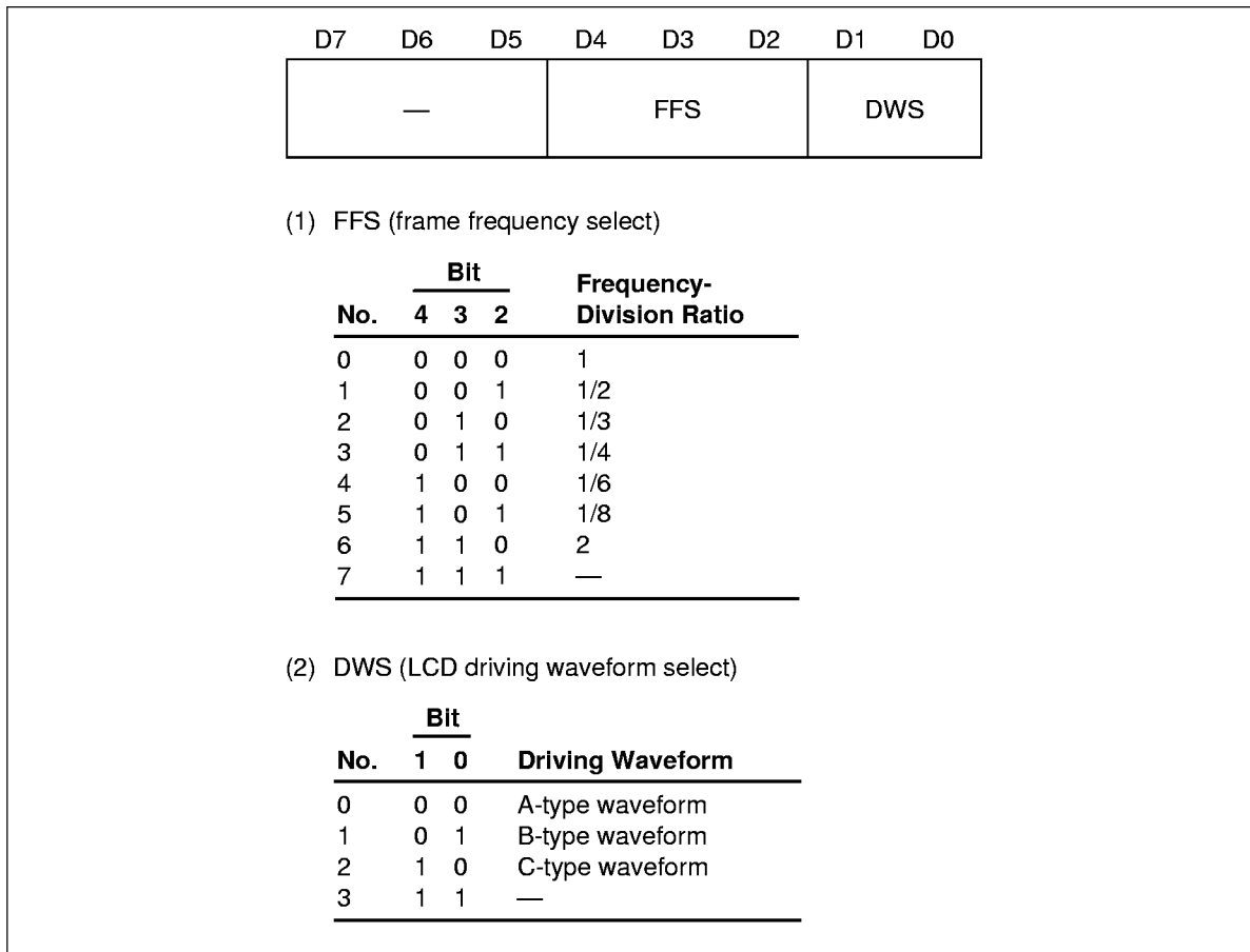
Figure 32 Mode Register
