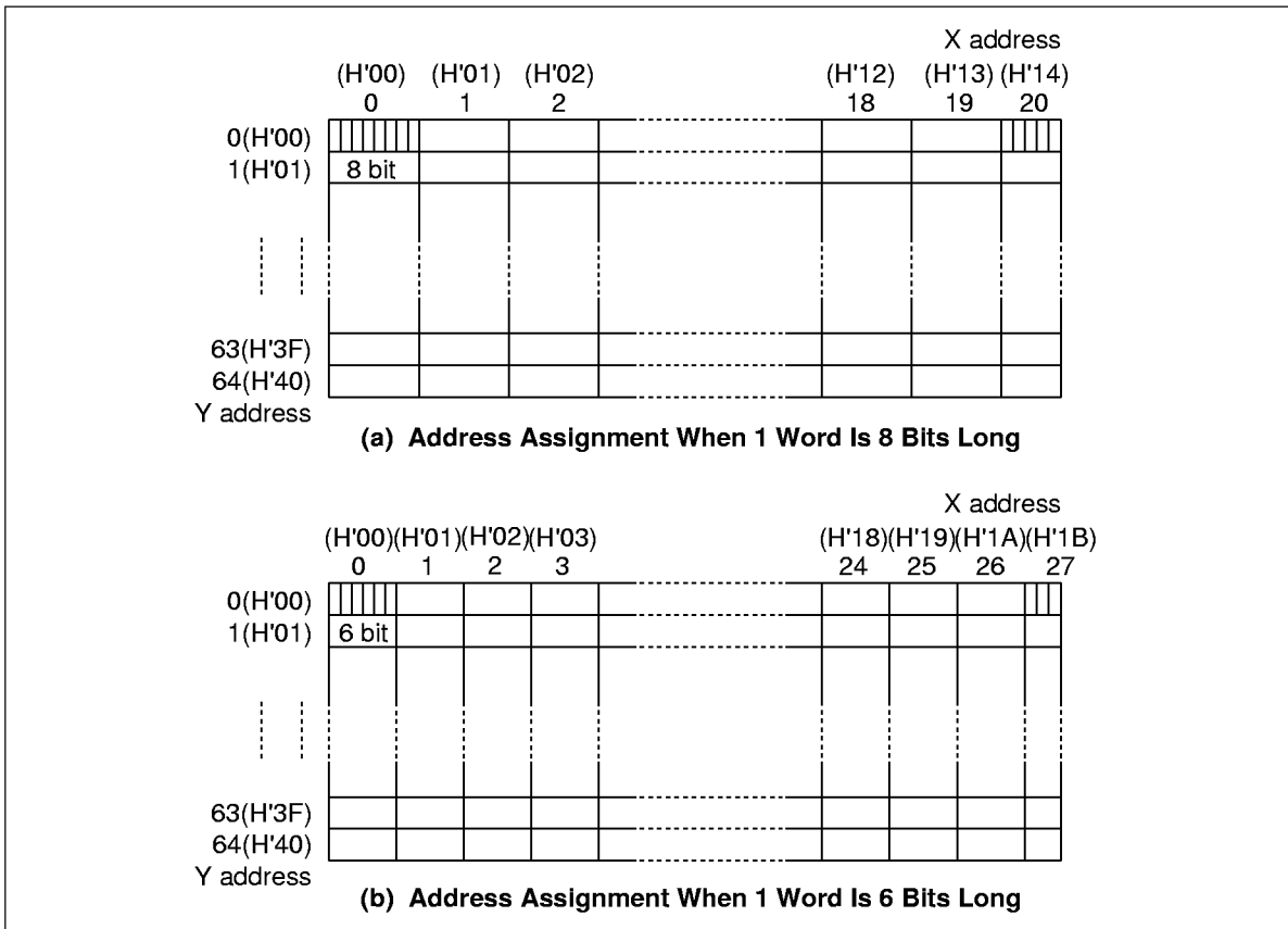
Figure 5 Display Memory Addresses
