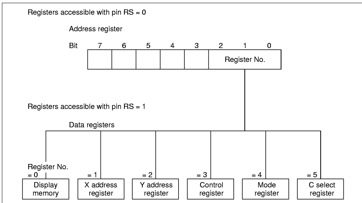
Figure 6 Relationship between Address Register and Register No.
