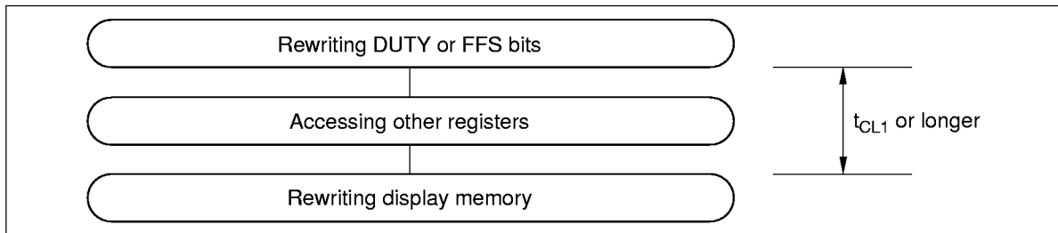
Figure 9 Rewriting Display Memory after Rewriting Registers
