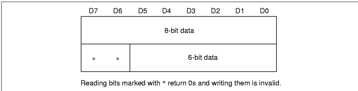
Figure 28 Display Memory
