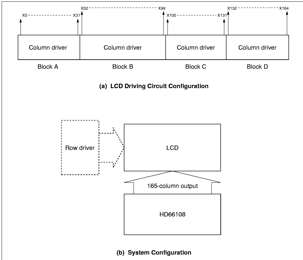
Figure 11 165-Column-Output Mode
