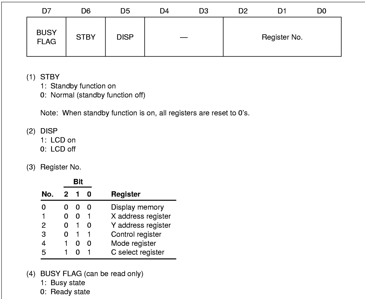
Figure 27 Address Register
