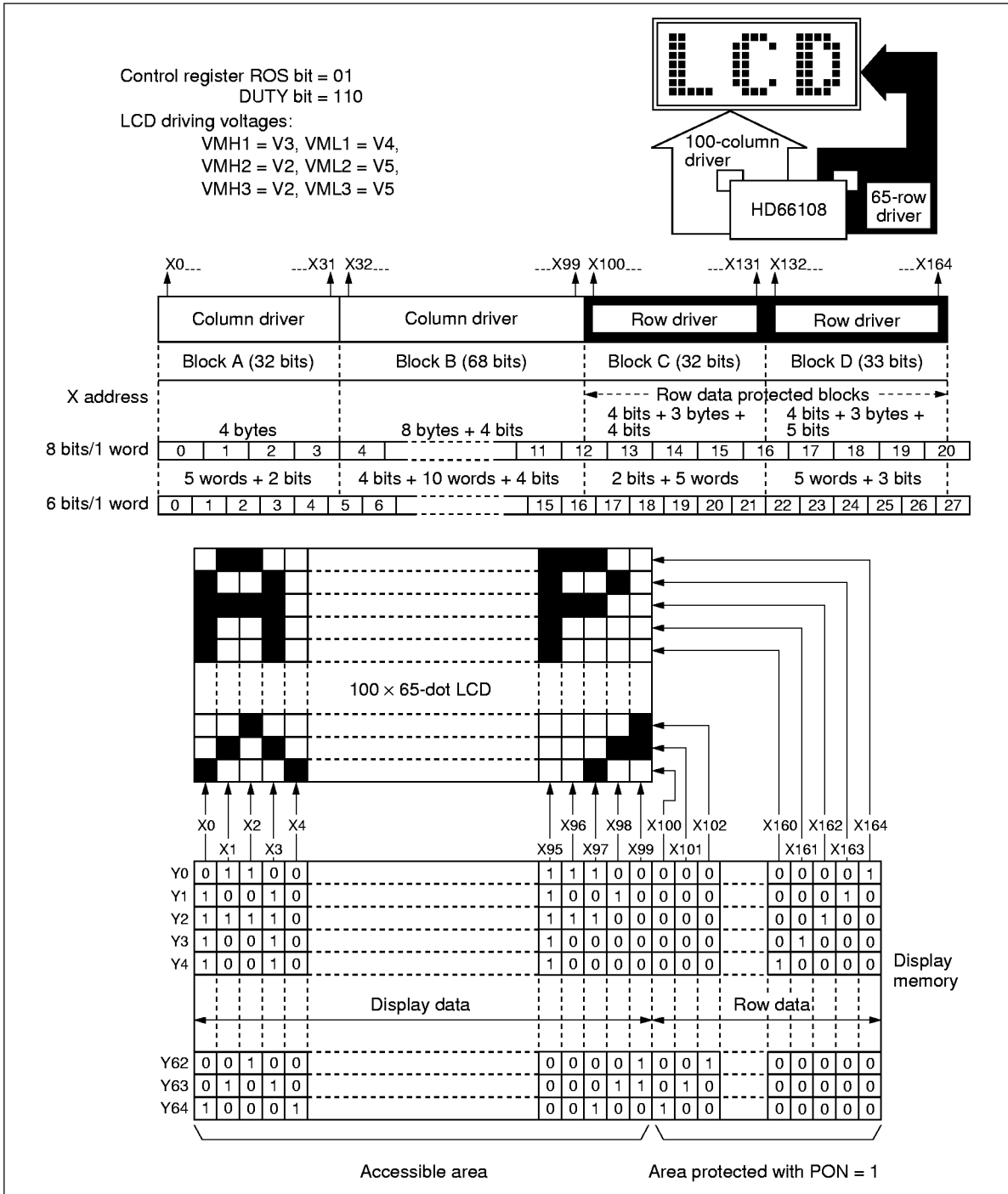
Figure 16 Relationship between Row Data and Display (65-Row Output from the Right Side, 1/66 Multiplexing Duty Ratio)
