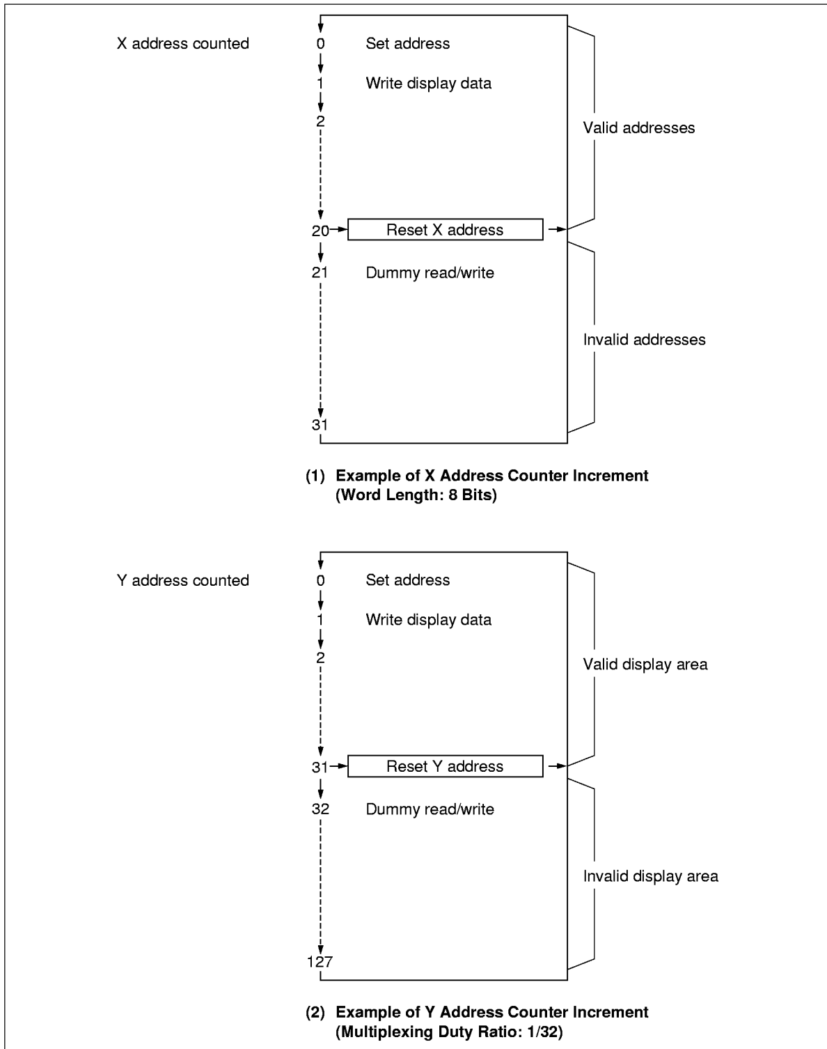
Figure 10 X/Y Address Counter Increment
