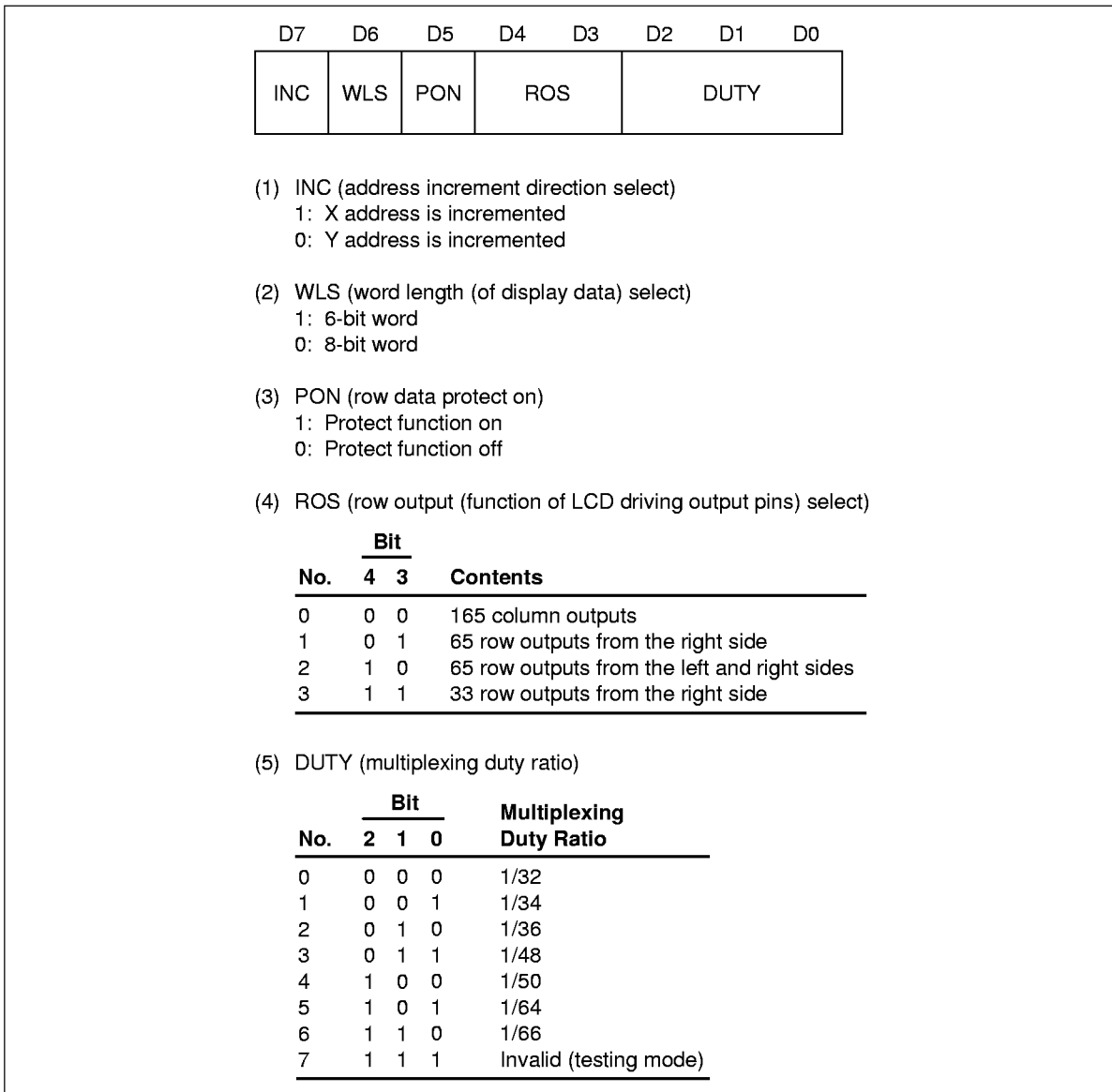
Figure 31 Control Register
