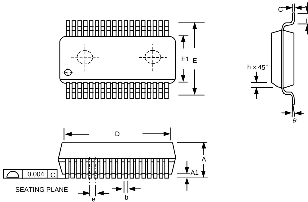
SSOP-36 Package
