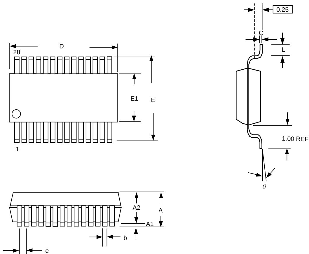
SSOP-28 Package
