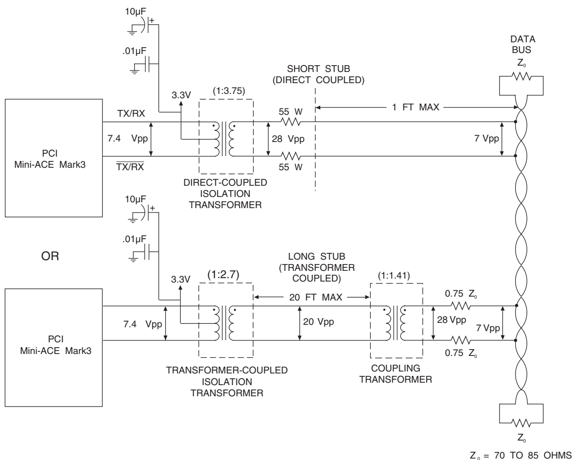
FIGURE 18. BU-65XXX8/9 (3.3V TRANSCEIVER) INTERFACE TO MIL-STD-1553 BUS
