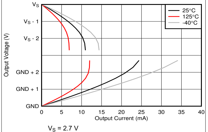
Figure 6-18. Output Voltage vs Output Current
