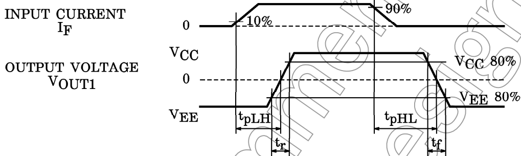
Fig.2 SWITCHING TIME TEST CONDITION
