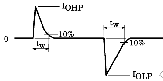
Fig.1 EXPONENTIAL WAVEFORM
