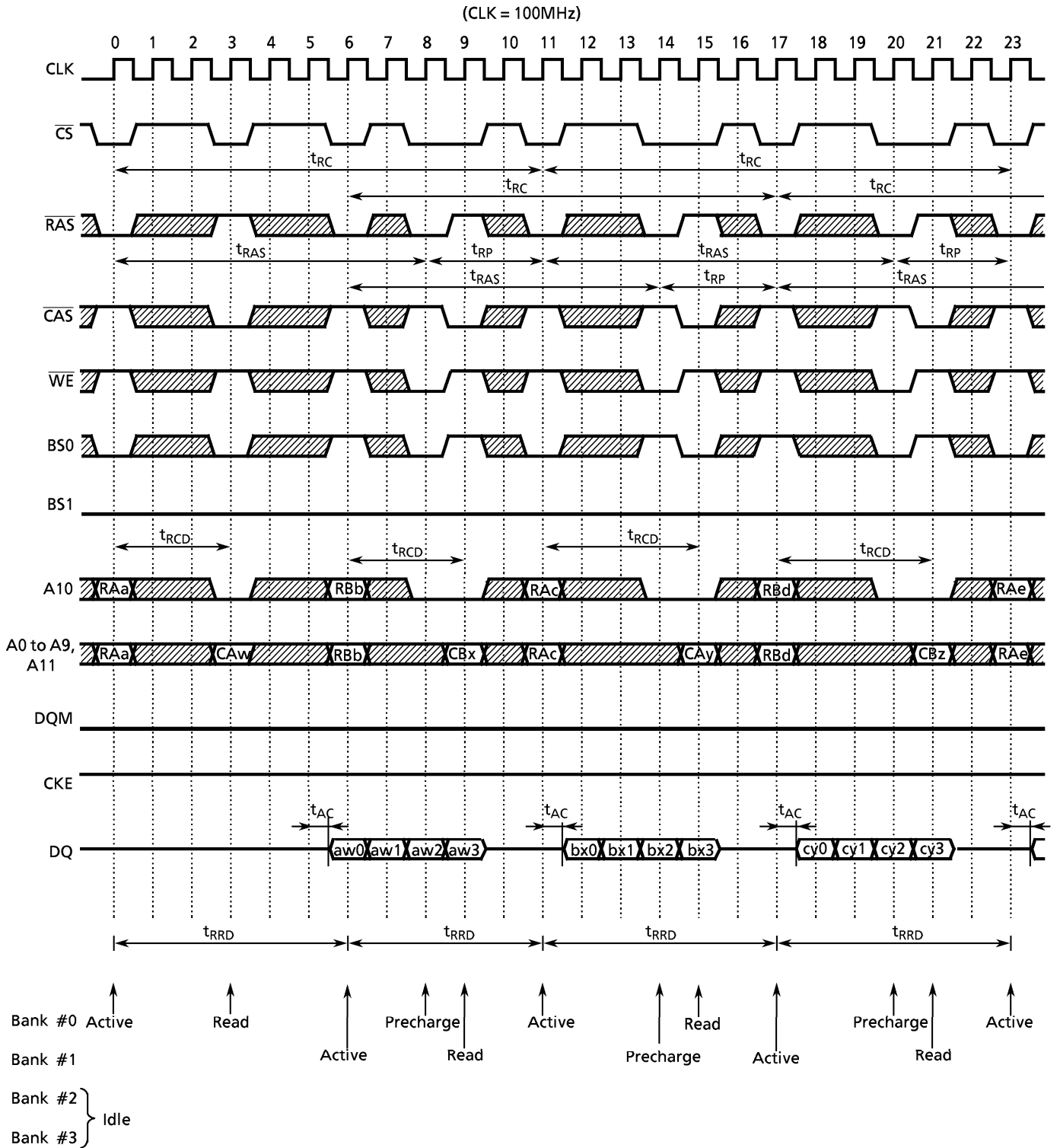
Figure 1. Interleaved Bank Read (Burst Length=4, \overline{\text{CAS}} Latency=3)
