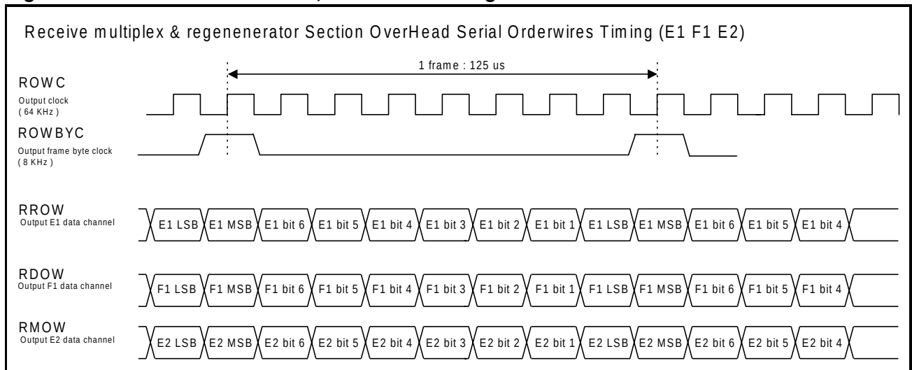
Figure 22: Receive Orderwire E1, F1 and E2 Timing
