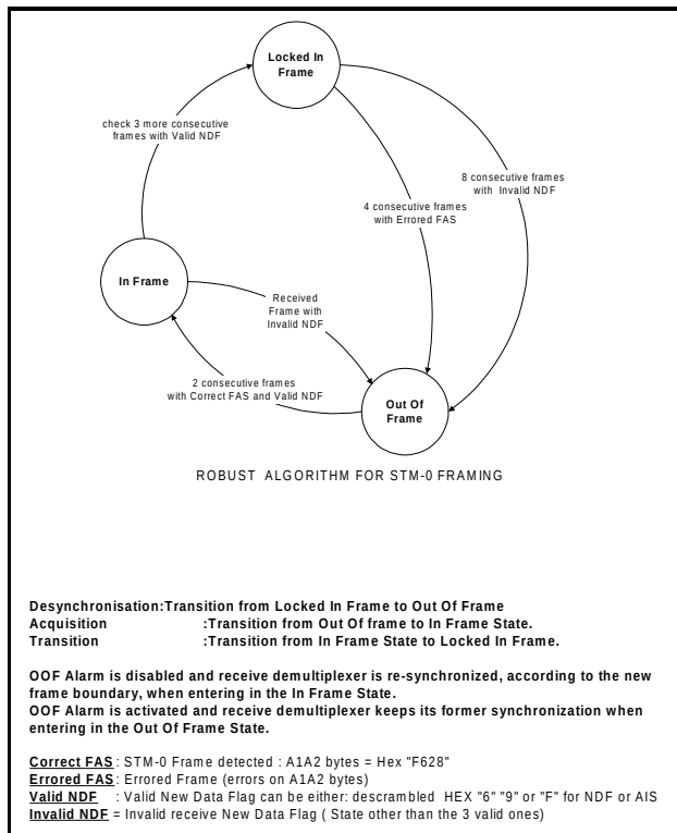
Figure 8: STM-0 Robust Frame State Machine
