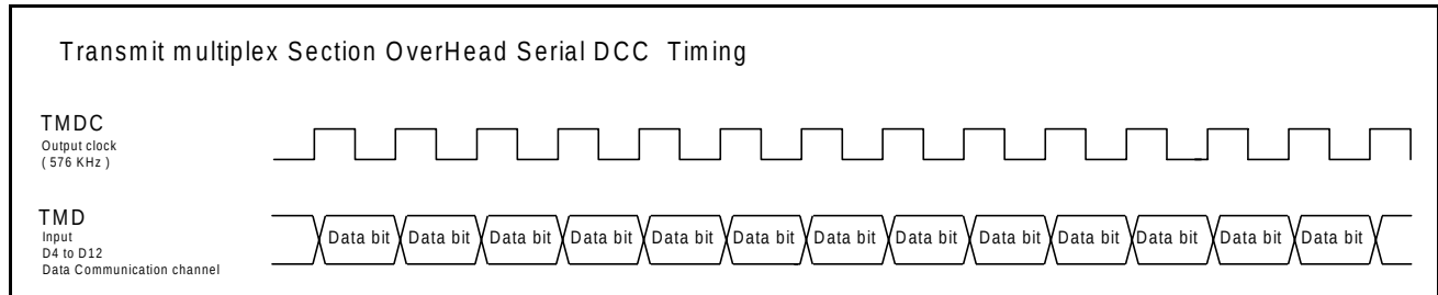
Figure 29: Transmit D4 to D12 Timing
