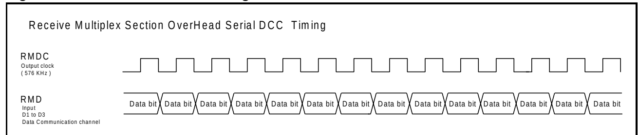
Figure 30: Receive D4 to D12 Timing
