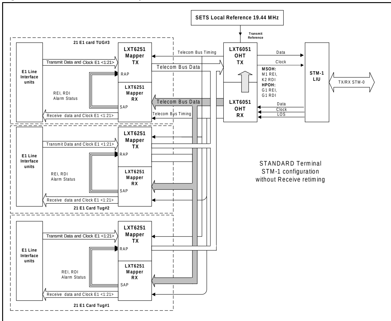
Figure 4: STM-1 Terminal Multiplexer
