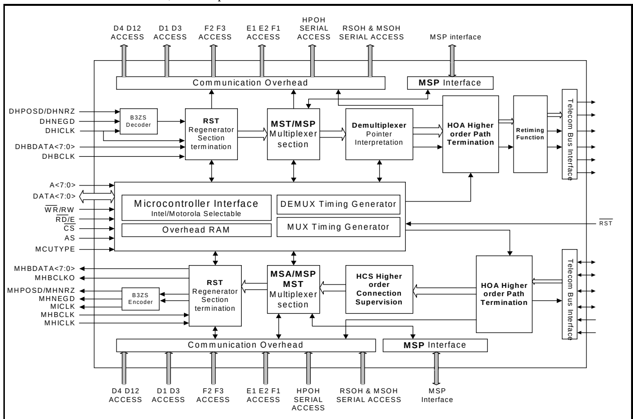
Figure 2: LXT6051 Block Diagram
