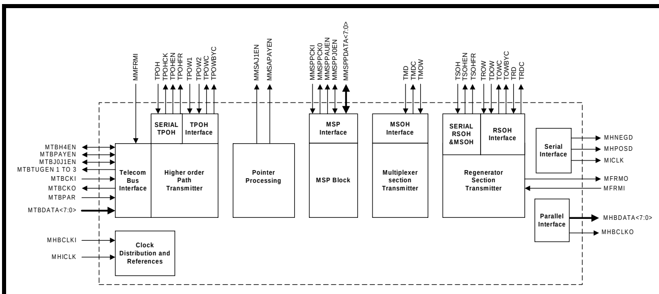
Figure 11: Transmit Detail Block Diagram
