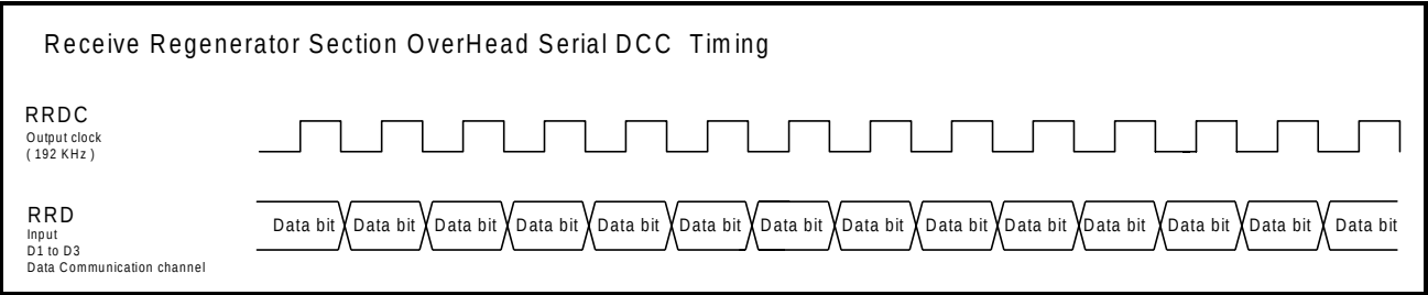
Figure 28: Receive D1 to D3 Timing
