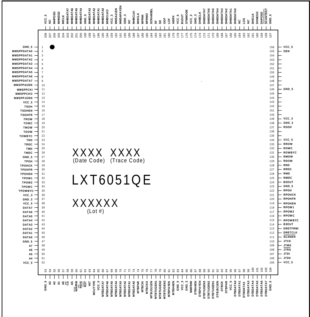
Figure 1: LXT6051 Pin Assignment
