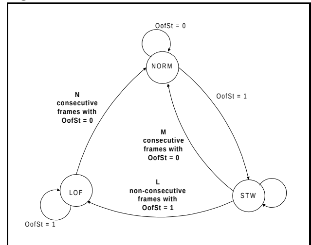
Figure 9: LOF State Machine
