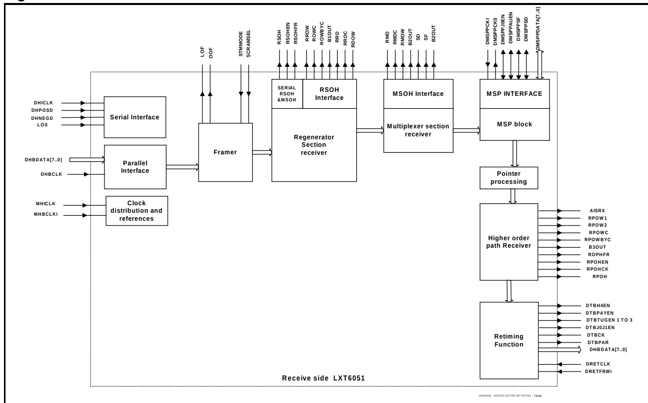
Figure 7: LXT6051 Receiver Blocks
