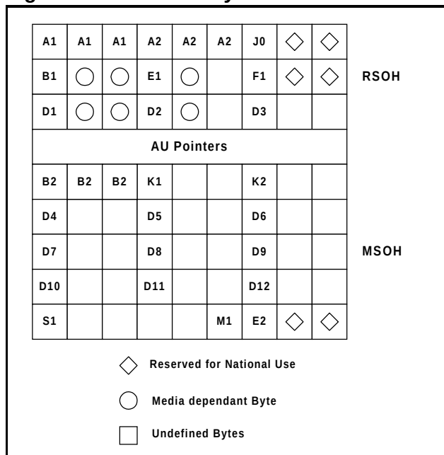
Figure 10: Overhead Bytes for the STM-1
