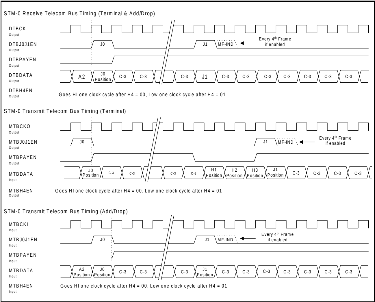
Figure 15: STM-0 Telecom Bus Timing
