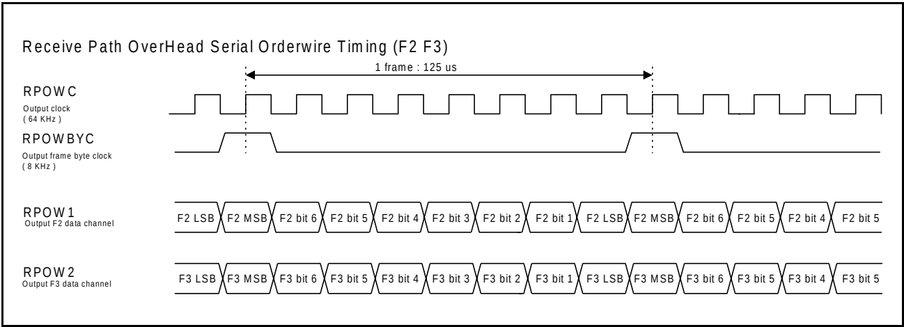
Figure 20: Receive F2 and F3 orderwire timing
