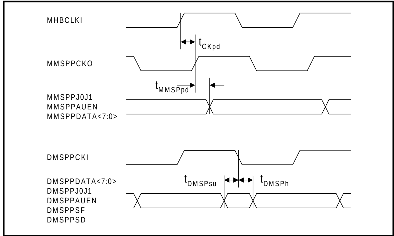
Figure 40: Master Mode MSP Bus Timing
