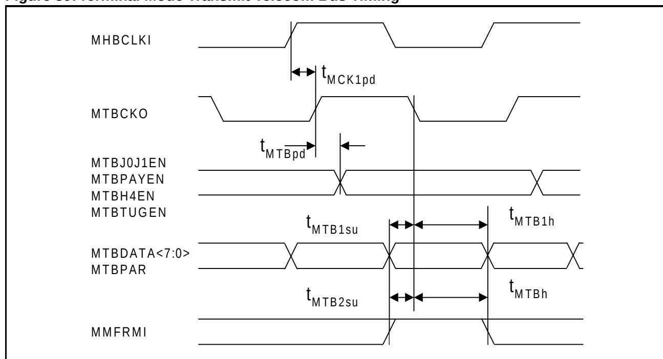
Figure 39: Terminal Mode Transmit Telecom Bus Timing
