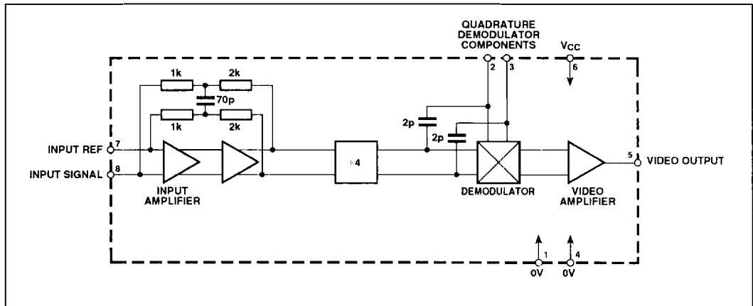
Fig. 2 Block diagram
