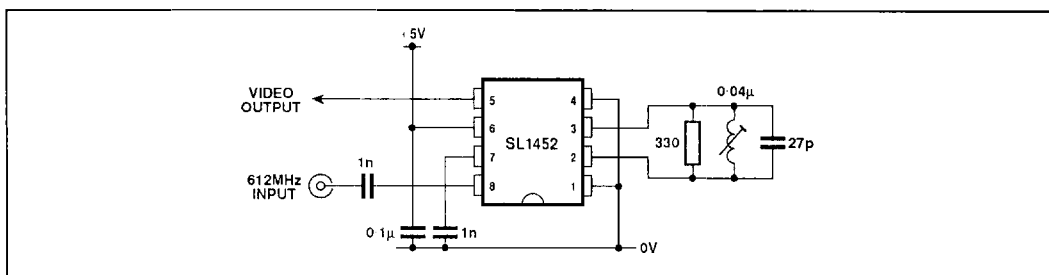
Fig. 4 Typical application
