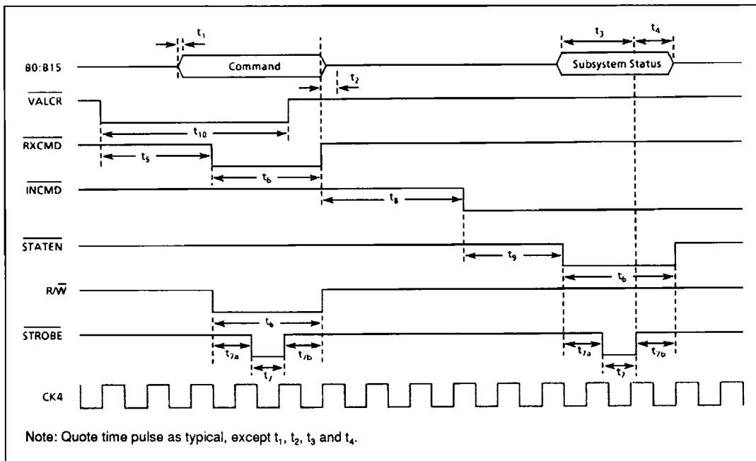
Figure 21: RT Command Reception and Subsystem Status Read
