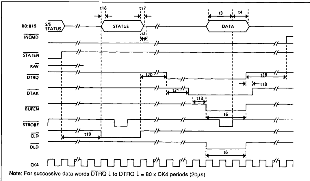
Figure 23: RT Status + RT-BC Data Transfer (Non Mode)
