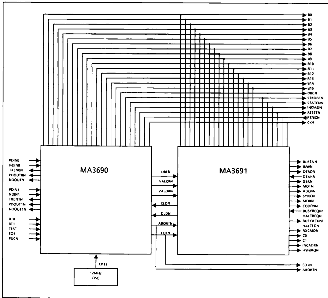
Figure 8: Chip Set Interconnection Diagram
