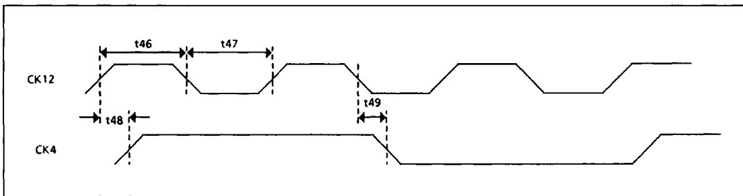
Figure 14: Clock Timing
