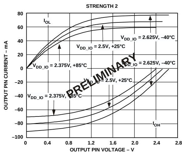
Figure 24. Typical Drive Currents at Strength 2
