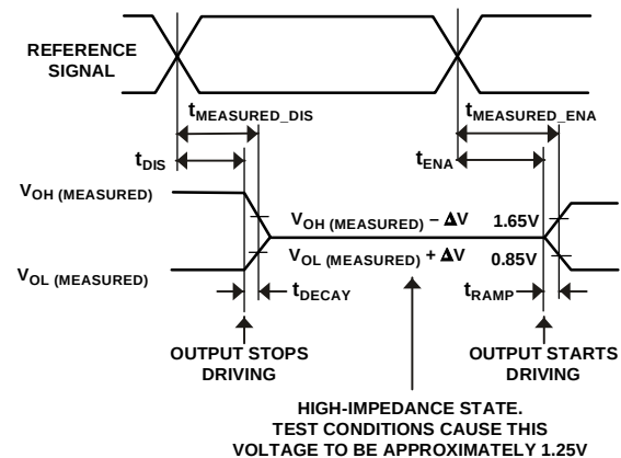
Figure 31. Output Enable/Disable
