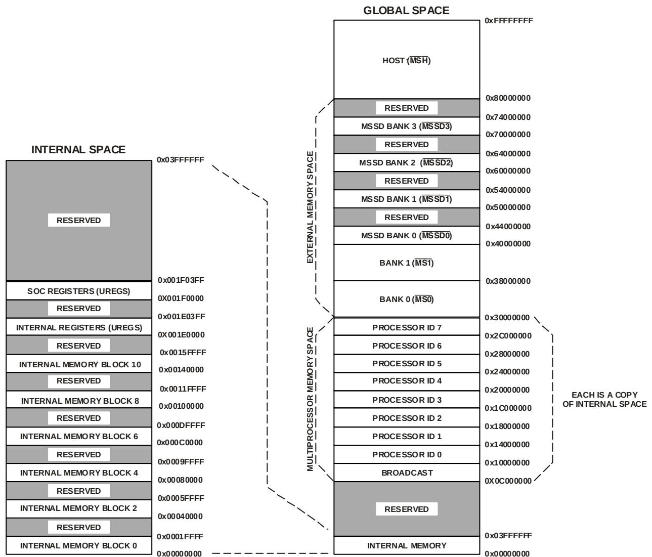
Figure 2. ADSP-TS201S Memory Map
