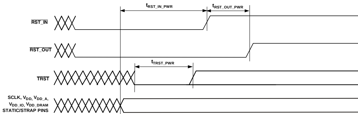
Figure 8. Power-Up Reset Timing
