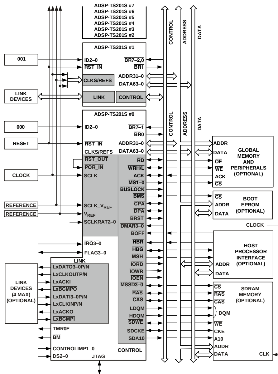
Figure 3. ADSP-TS201S Shared Memory Multiprocessing System
