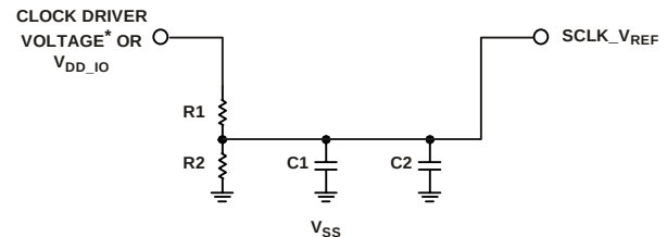
Figure 5. V_{REF} filtering scheme
