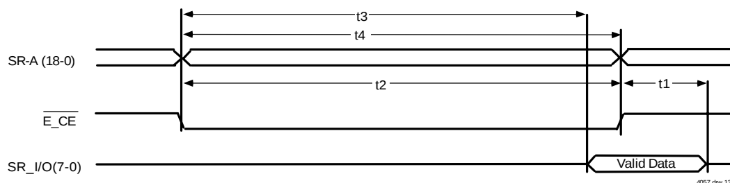
Figure 8 EPROM Timing
