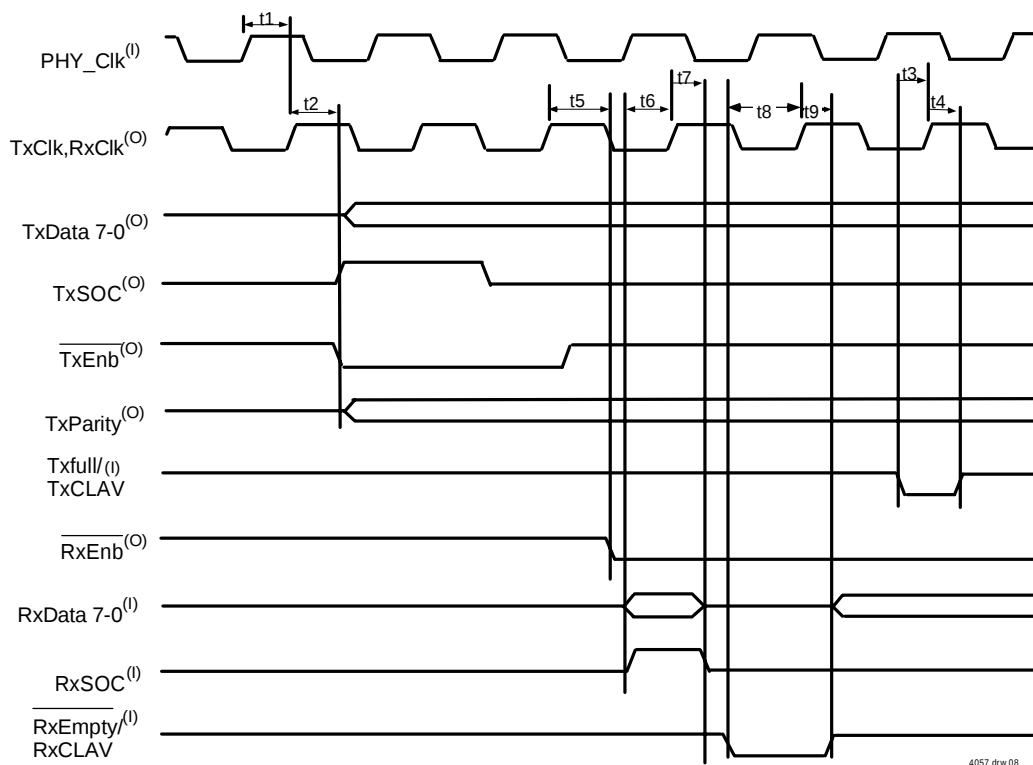
Figure 3 UTOPIA Bus Timing
