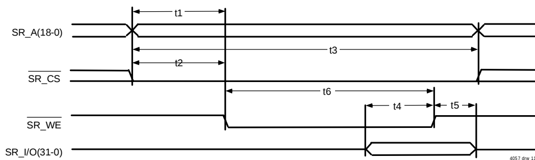
Figure 6 SRAM Bus Write Cycle Timing
