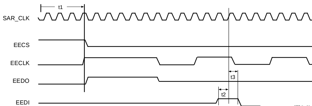
Figure 9 EEPROM Timing
