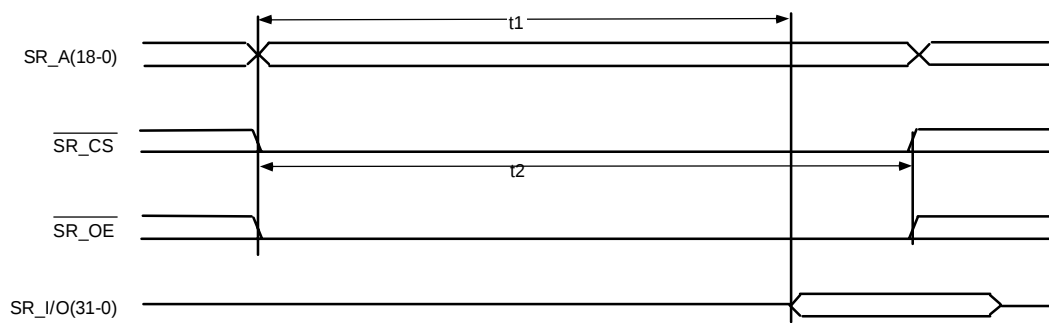
Figure 7 SRAM Bus Read Cycle Timing
