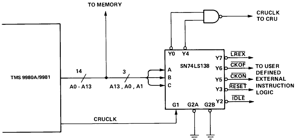
FIGURE 7 – EXTERNAL INSTRUCTION DECODE LOGIC
