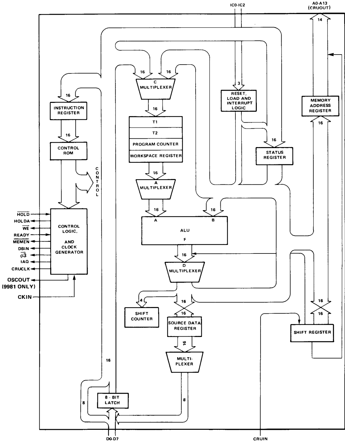
FIGURE 1 - ARCHITECTURE
