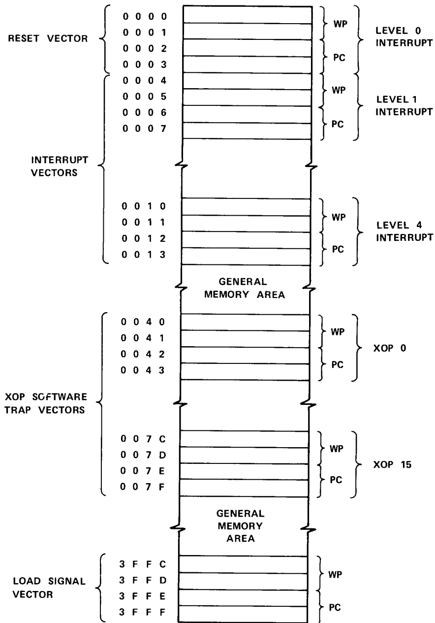
FIGURE 2 – MEMORY MAP
