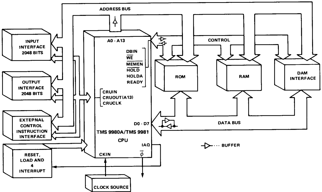
FIGURE 16 - MAXIMUM TMS 9980 SYSTEM
