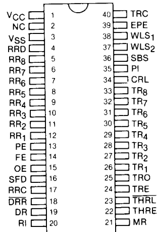
PIN DESIGNATION
