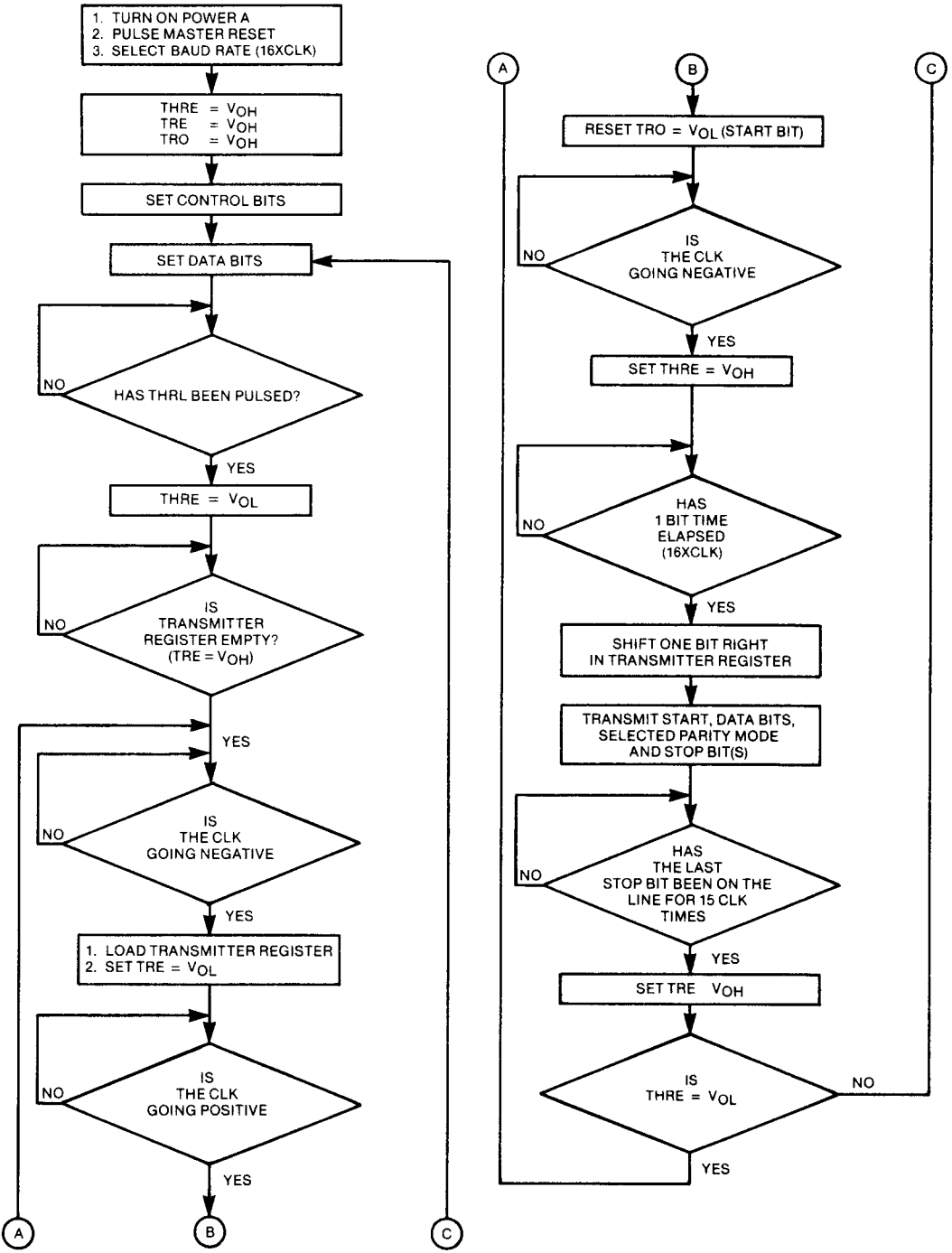
TRANSMITTER FLOW CHART
