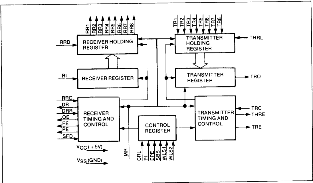
TR1863/TR1865 BLOCK DIAGRAM
