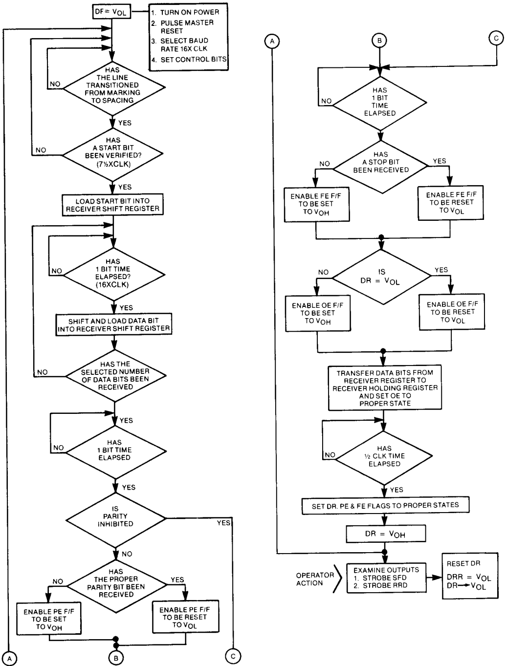
RECEIVER FLOW CHART
