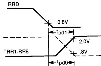
*RR1-RR3 ARE DISCONNECTED AT TRANSITION OF RRD FROM 0.8V TO 2.0V.
