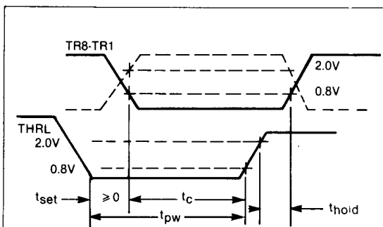
FIGURE 2. DATA INPUT LOAD CYCLE
