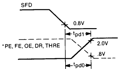
*PE, FE, OE, DR, THRE ARE DISCONNECTED AT TRANSITION OF SFD FROM 0.8V TO 2.0V.
