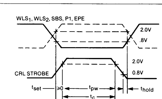
FIGURE 3. CONTROL REGISTER LOAD CYCLE
