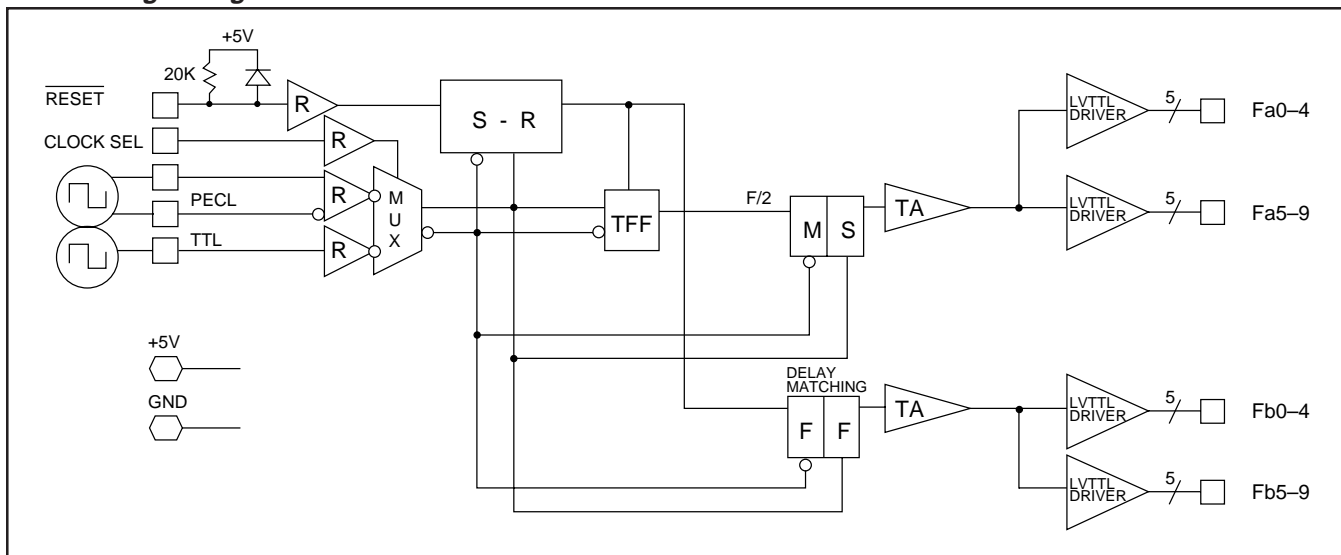
SC3306 Logic Diagram
