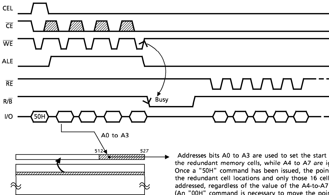
Figure 5. Read mode (3) operation
