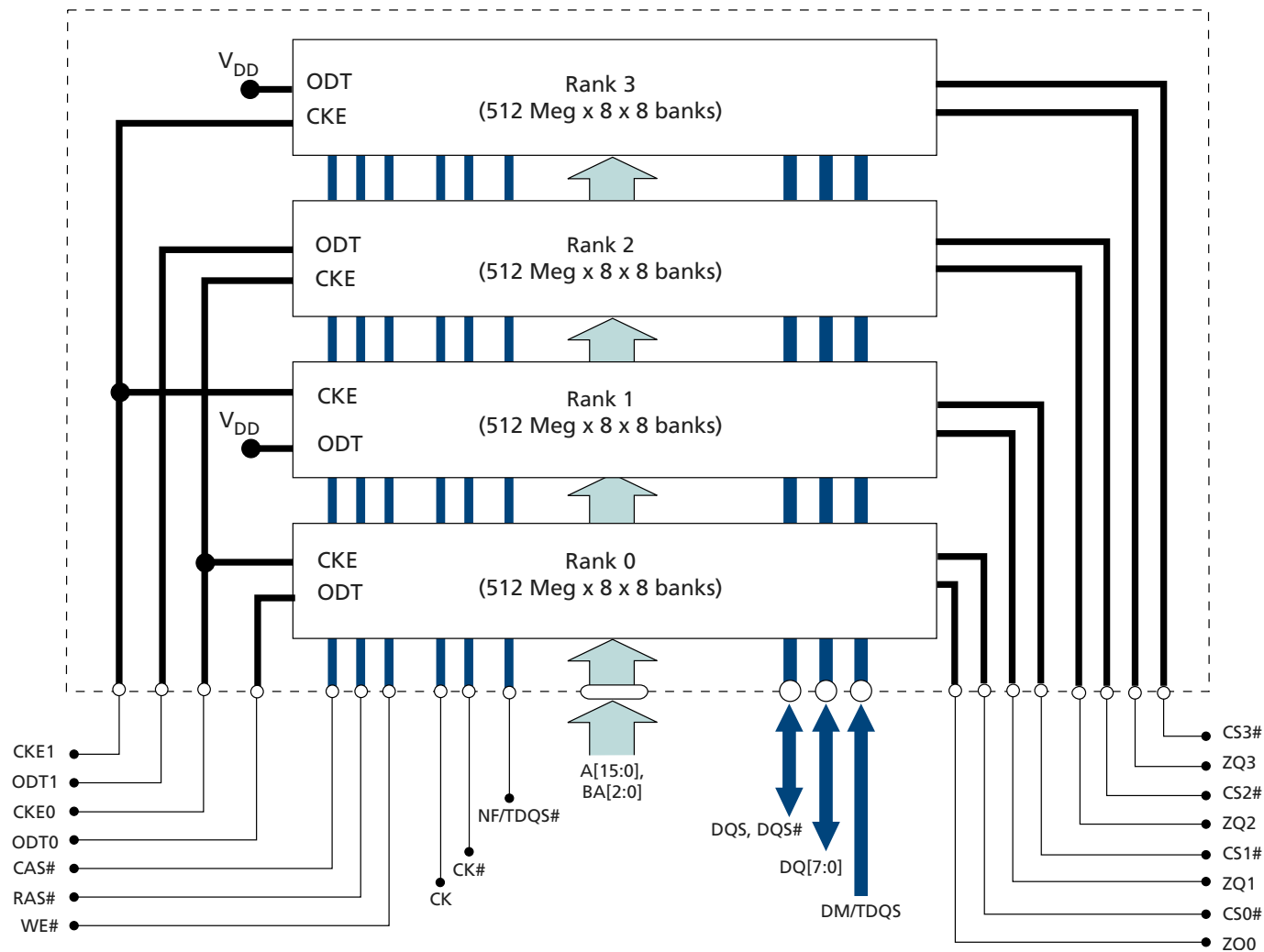
Figure 3: Functional Block Diagram (512 Meg x 8 x 8 Banks x 4 Ranks)
