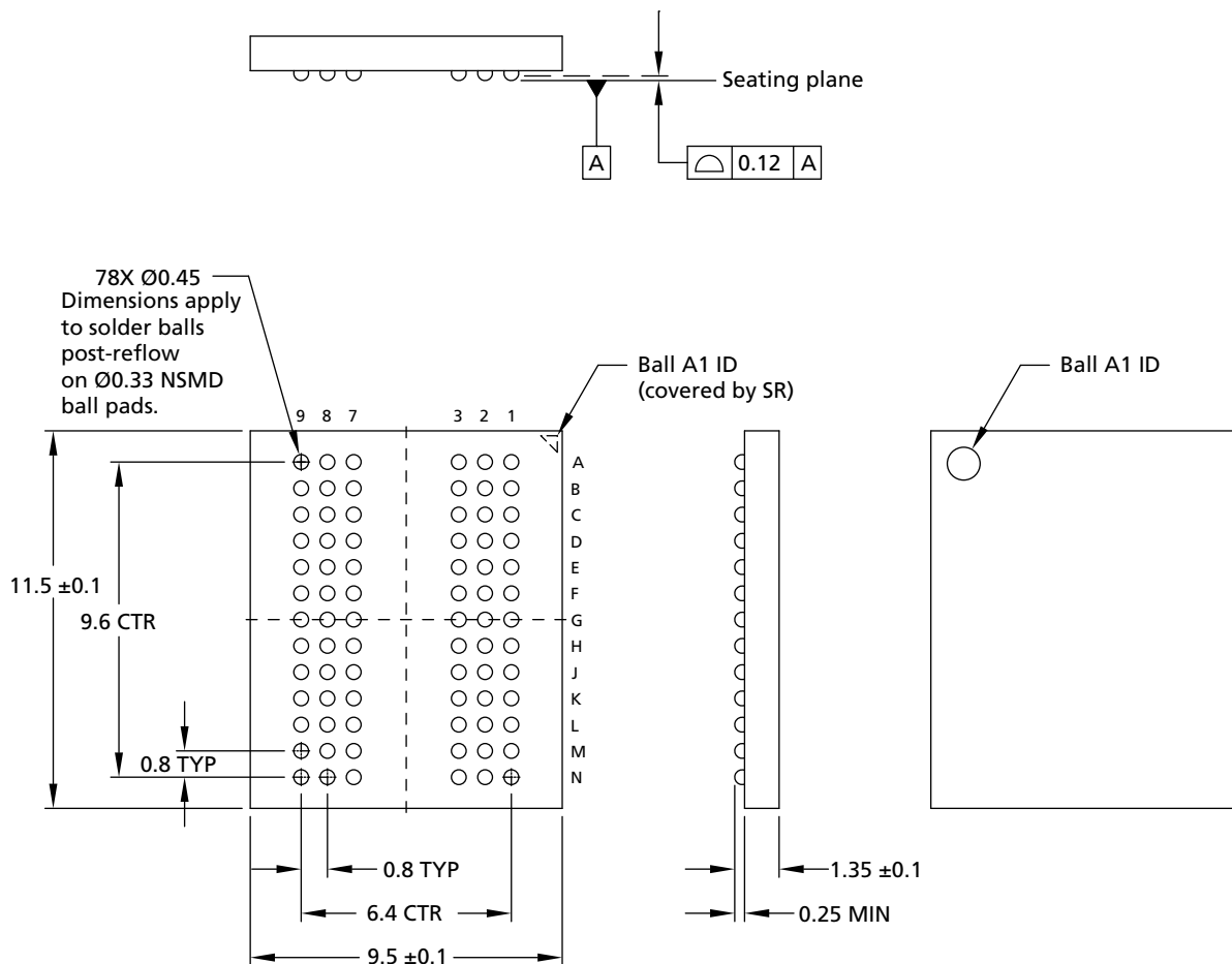
Figure 5: 78-Ball FBGA (package code SMA)
