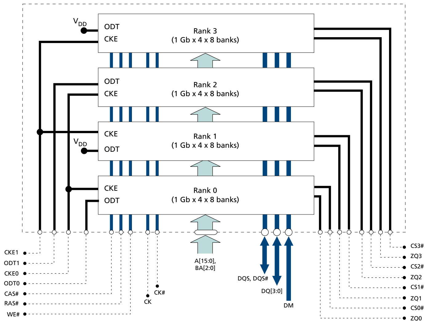
Figure 2: Functional Block Diagram (1 Gb x 4 x 8 Banks x 4 Ranks)
