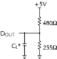
Figure 1. Output Load * Including Probe and Jig Capacitance.
