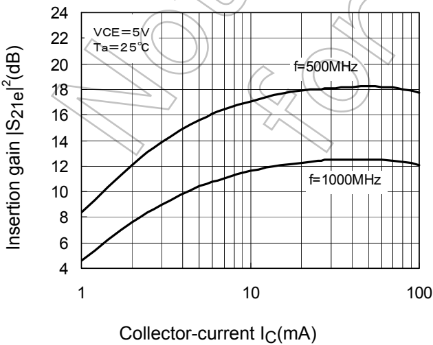
|S_{21e}|^2-I_C
