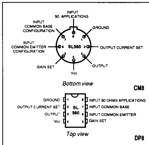
Fig. 1 Pin connections
