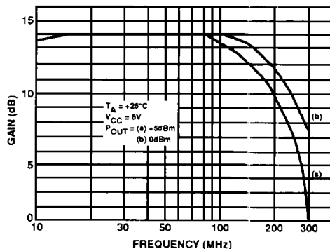
Fig.4 Frequency response, small signal gain is of a typical device
