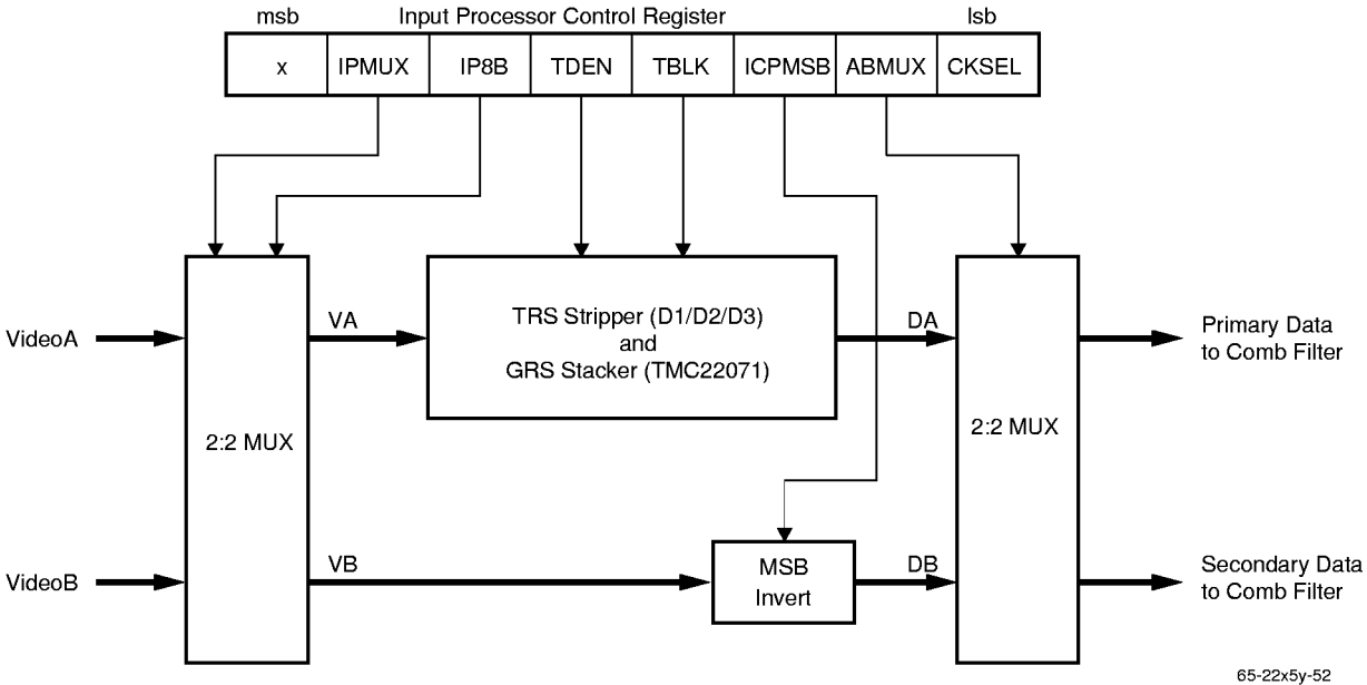
Figure 11. Input Processor
