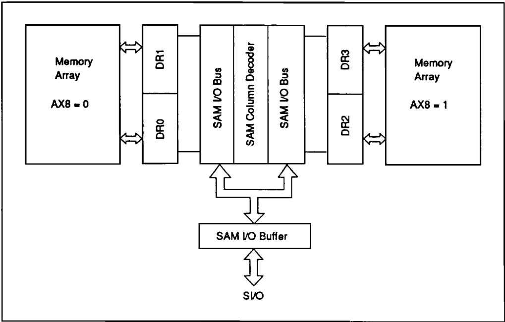
Figure 4 Block Diagram for Split Transfer
