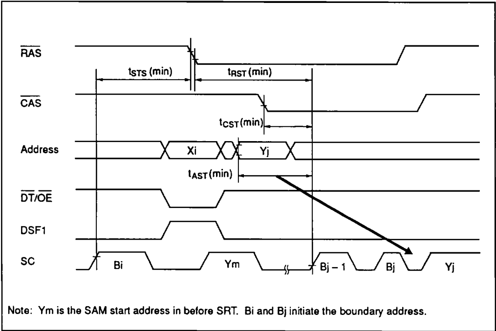
Figure 5 Limitation in Split Transfer
