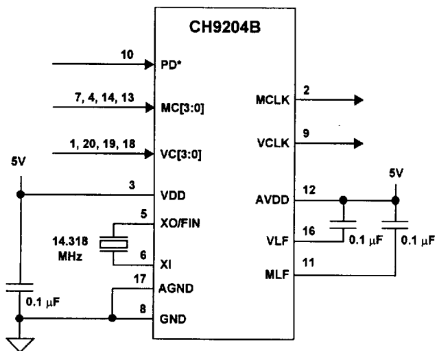
Figure 3: Application Schematic
