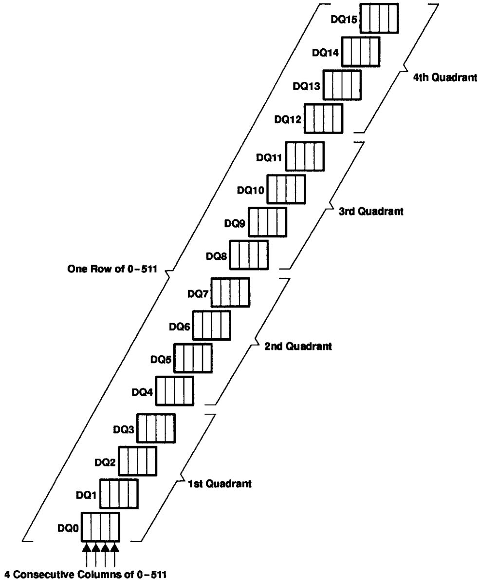
Figure 8. Block-Write Operation
