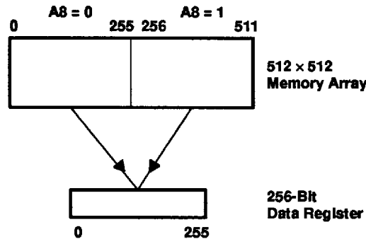
Figure 14. Full-Register-Transfer Read
