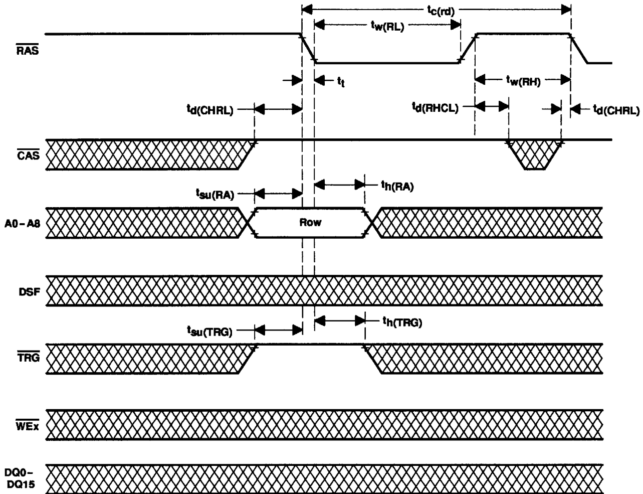
Figure 42. RAS-Only Refresh-Cycle Timing
