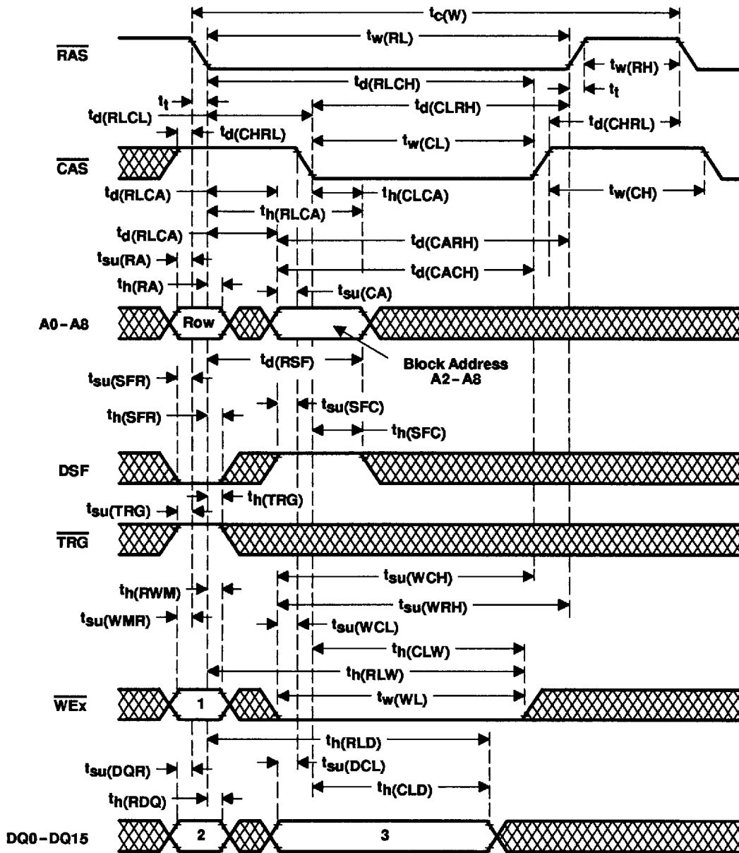
Figure 39. Block-Write-Cycle Timing (Early Write)
