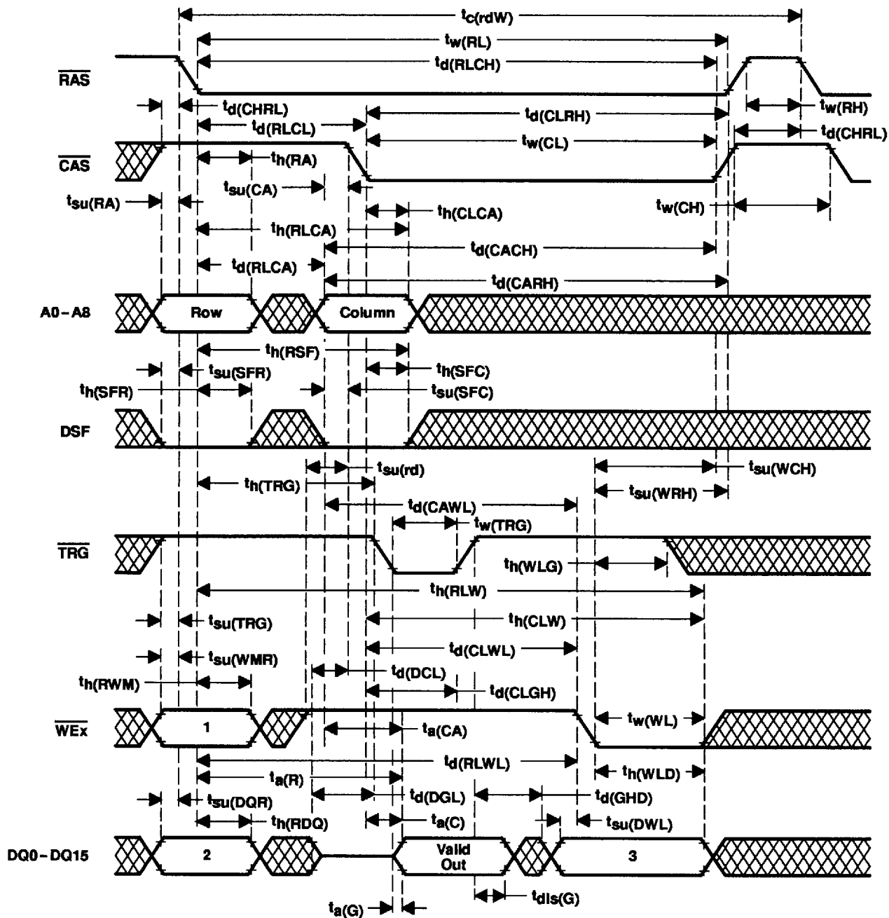
Figure 32. Read-Write-/Read-Modify-Write-Cycle Timing
