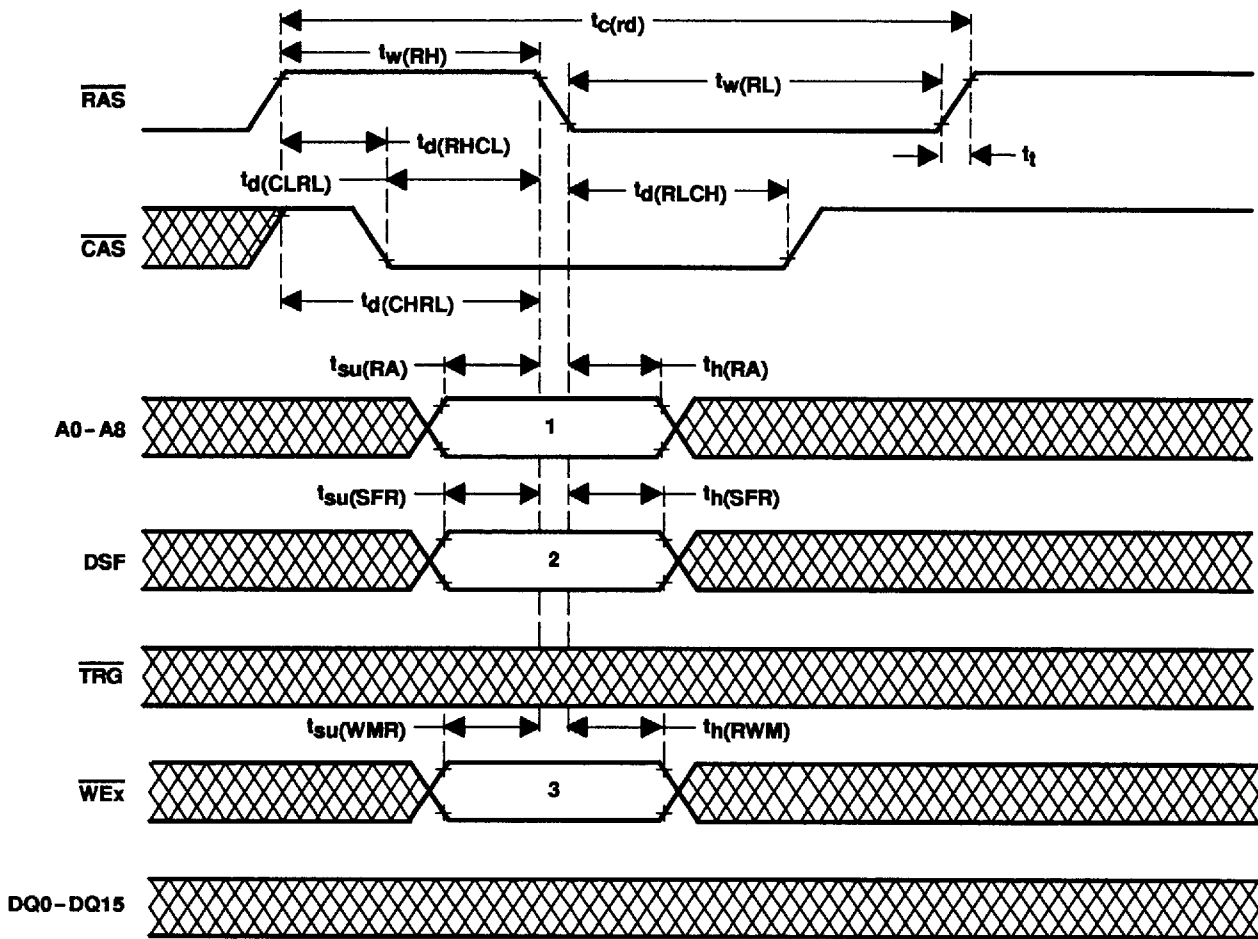
Figure 43. CBR-Refresh-Cycle Timing
