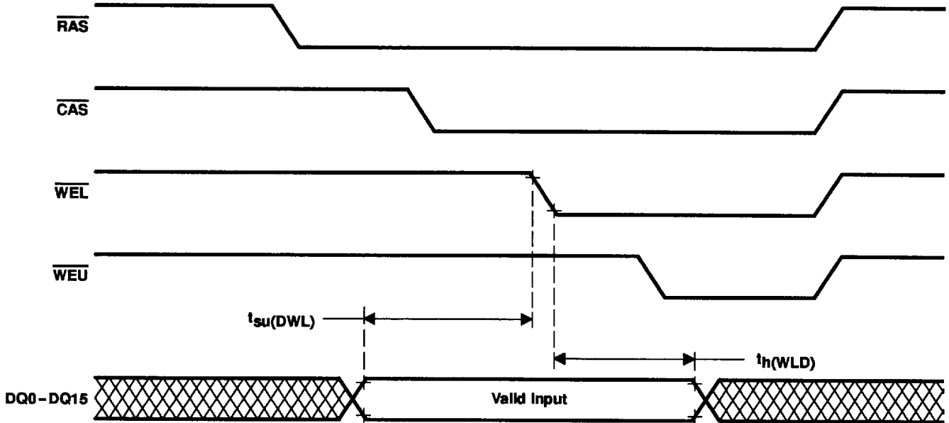
Figure 5. Example of a Late-Write Cycle
