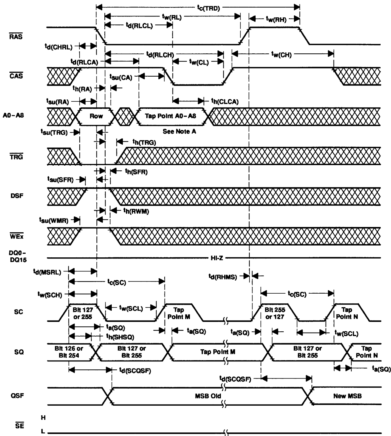
Figure 47. Split-Register-Transfer Read Timing
