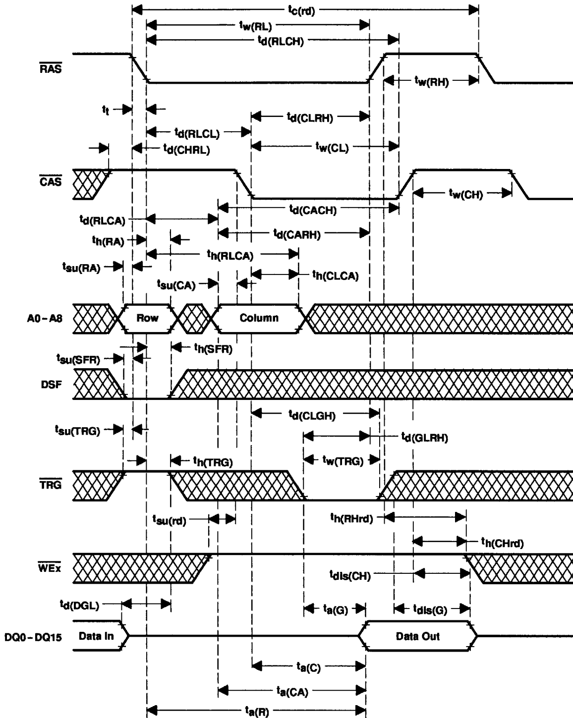
Figure 26. Read-Cycle Timing With CAS-Controlled Output
