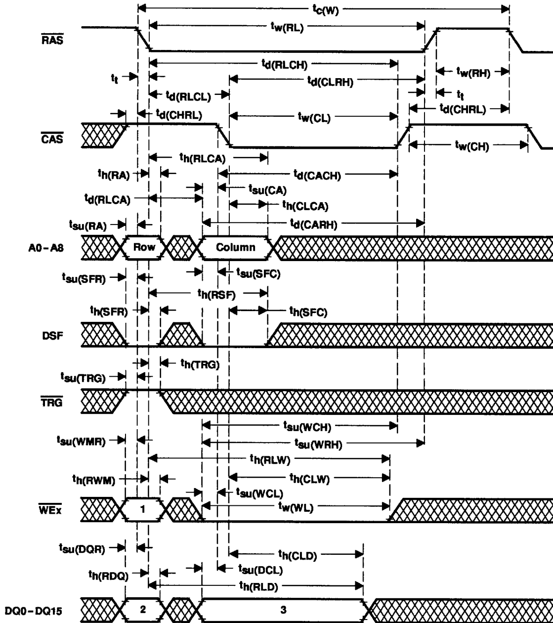
Figure 28. Early-Write-Cycle Timing
