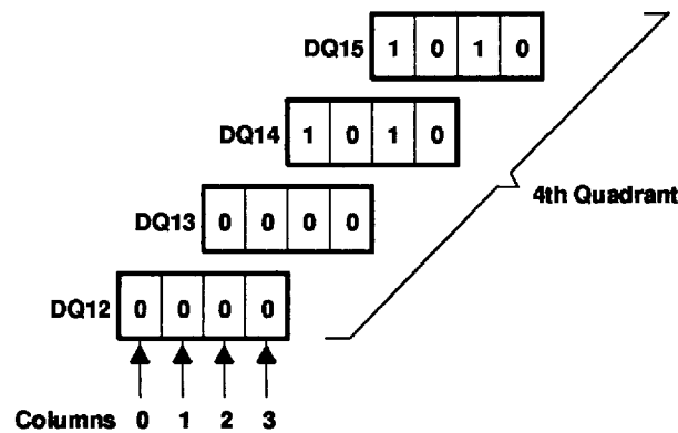
Figure 11. Example of Fourth Quadrant After Block-Write Operation
