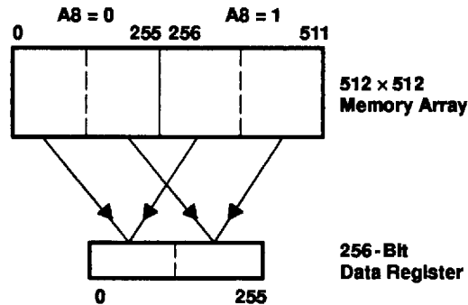
Figure 16. Split-Register-Transfer Read
