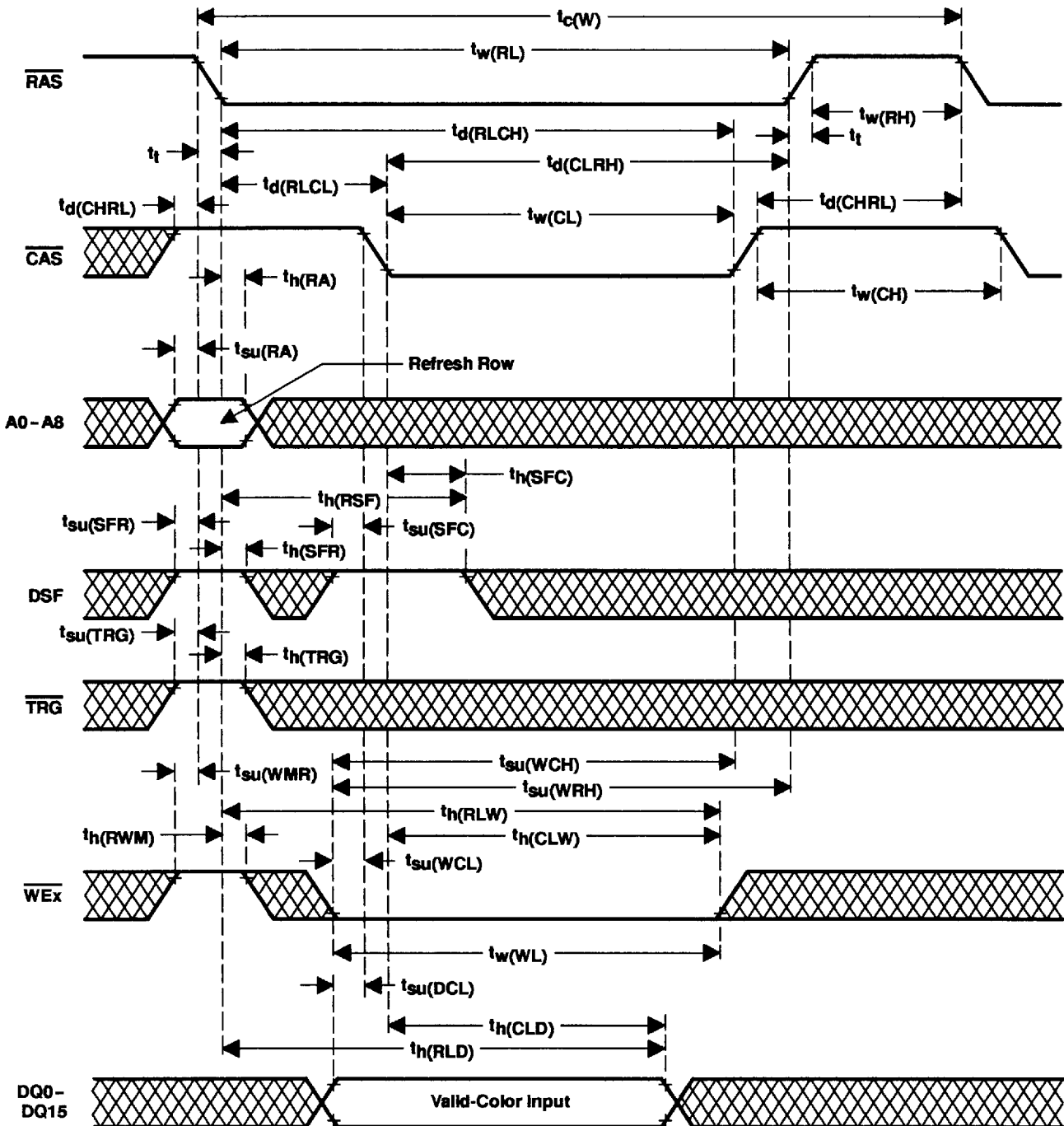
Figure 37. Load-Color-Register-Cycle Timing (Early-Write Load)
