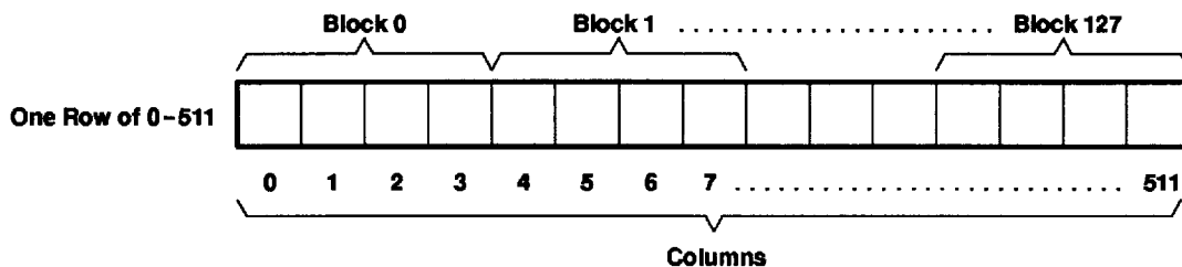
Figure 10. Block Columns Organization
