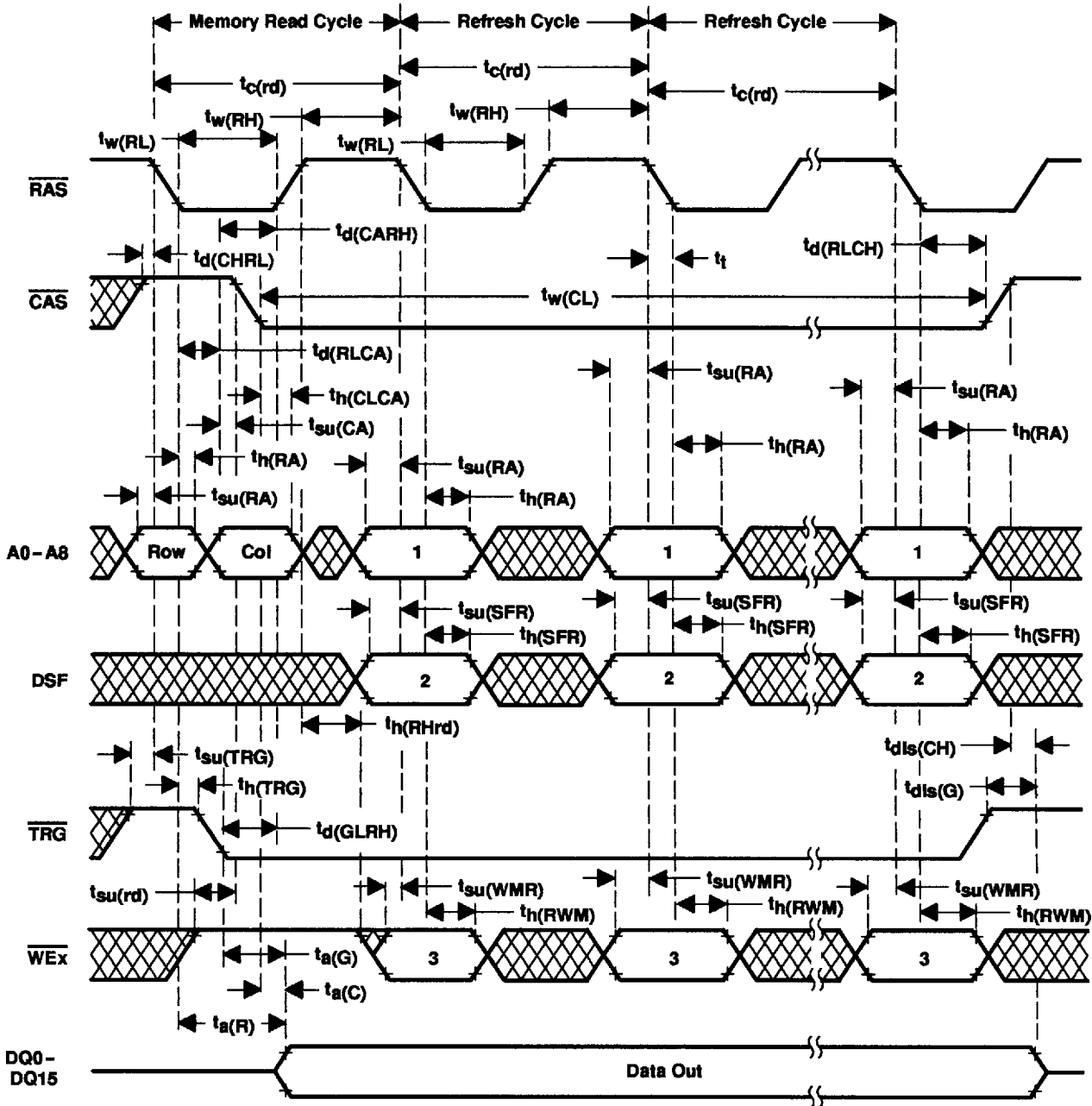
Figure 44. Hidden-Refresh-Cycle Timing
