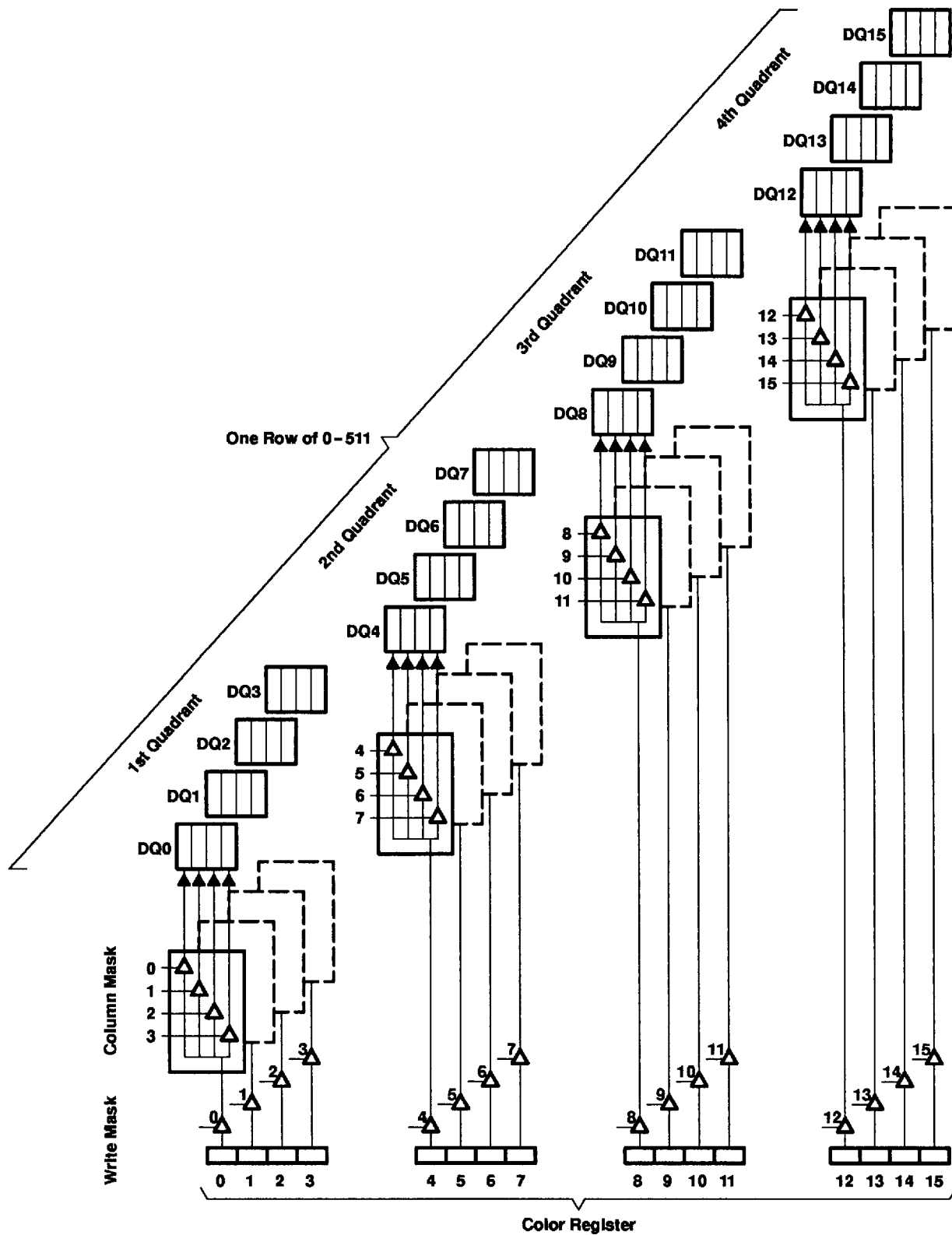
Figure 9. Block Write With Masks
