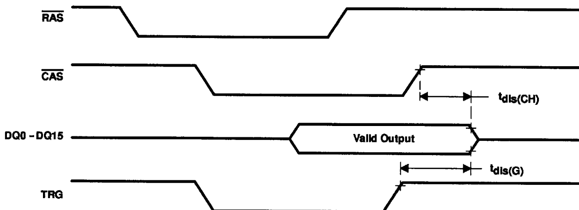
Figure 2. DRAM Read Cycle With \overline{\text{CAS}} -Controlled Output
