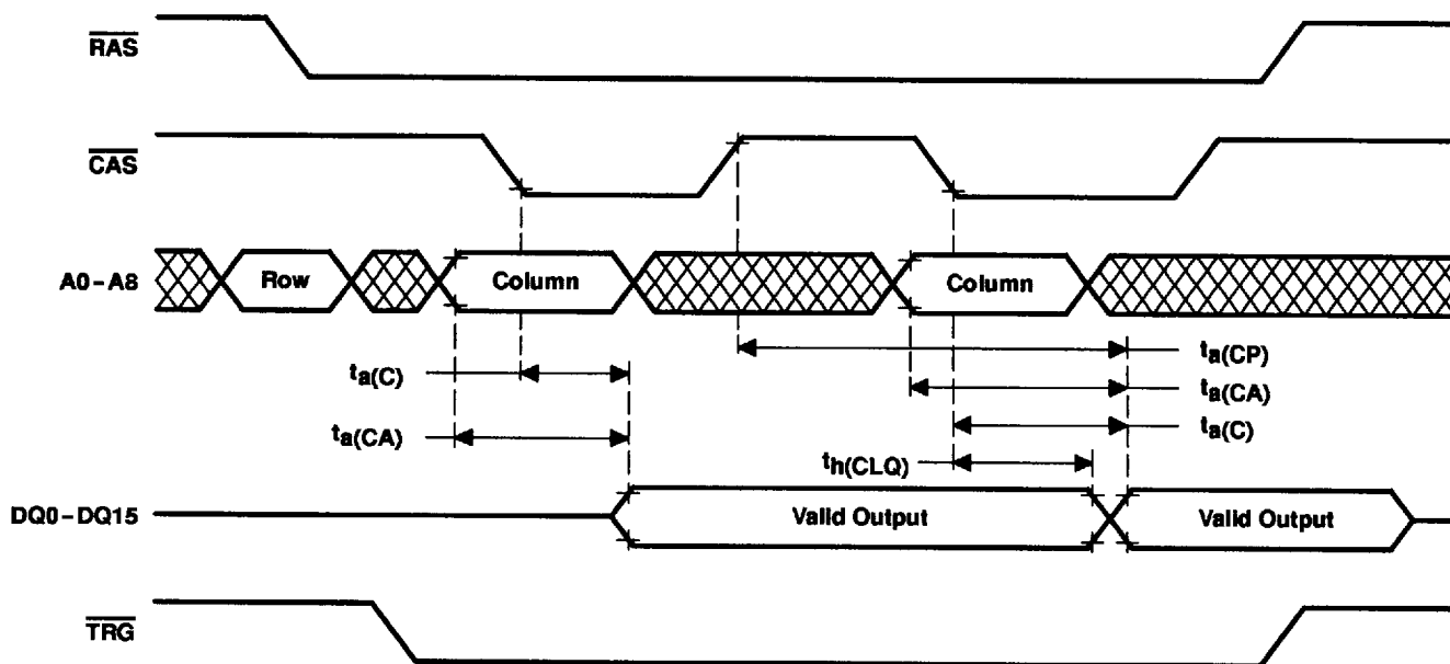
Figure 3. DRAM Page-Read Cycle With Extended Output
