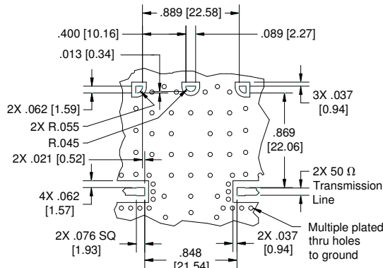
Dimensions are in Inches [Millimeters] XDL20-11-180 Rev A Mounting Footprint
