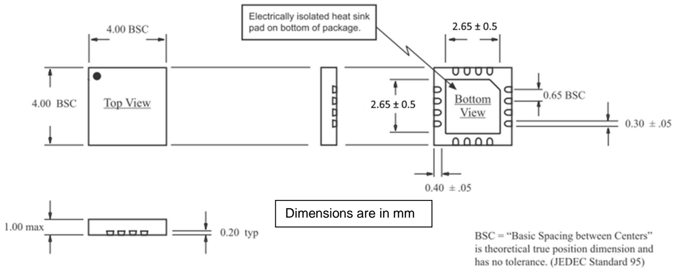
Figure 6 16L QFN 4x4 G Package Outline
