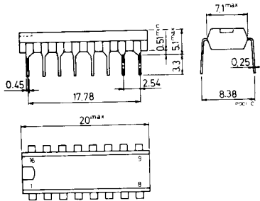
Dual in-line plastic package
