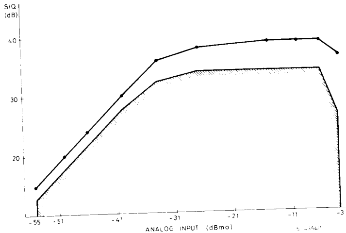
Fig. 2 - S/Q ratio vs. input level.
