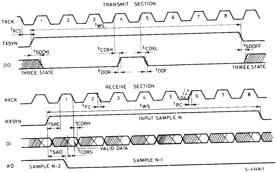
Fig. 1 - Transmit and receive sections
