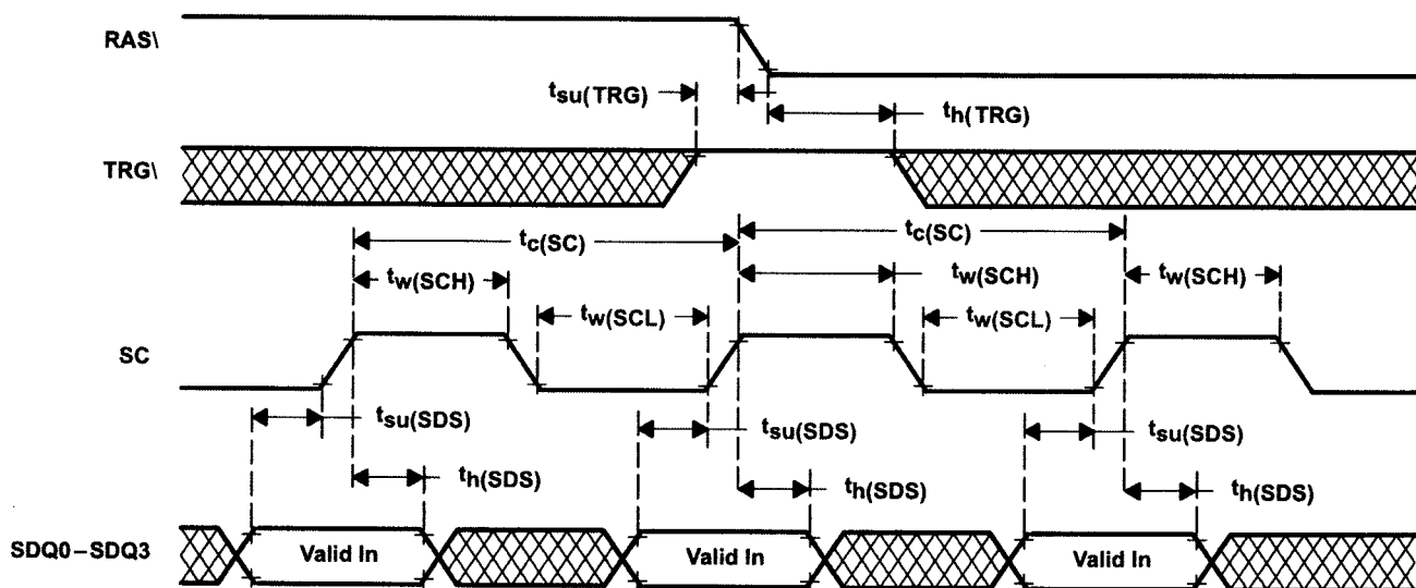
FIGURE 36: Serial-Write-Cycle Timing ( SE\downarrow = V_{IL} )
