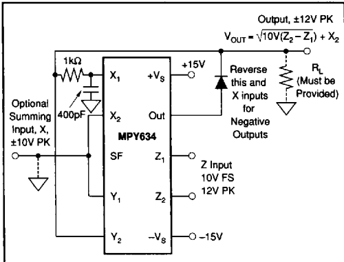
FIGURE 5. Square-Rooter Connection.
