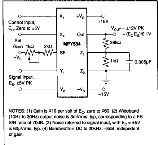
FIGURE 7. Voltage-Controlled Amplifier.
