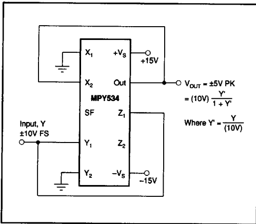
FIGURE 11. Bridge-Linearization Function.
