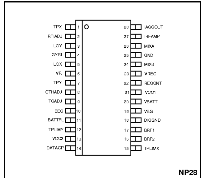
Fig.1 Pin connections
