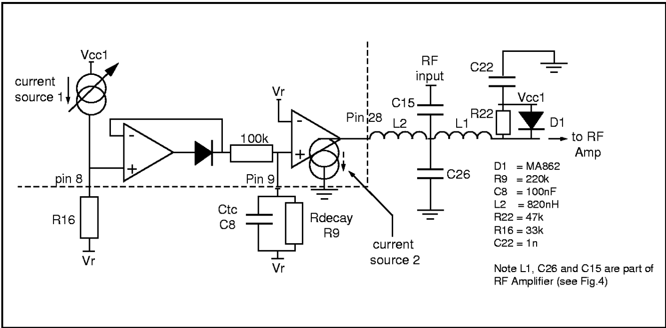
Fig.6 AGC Schematic
