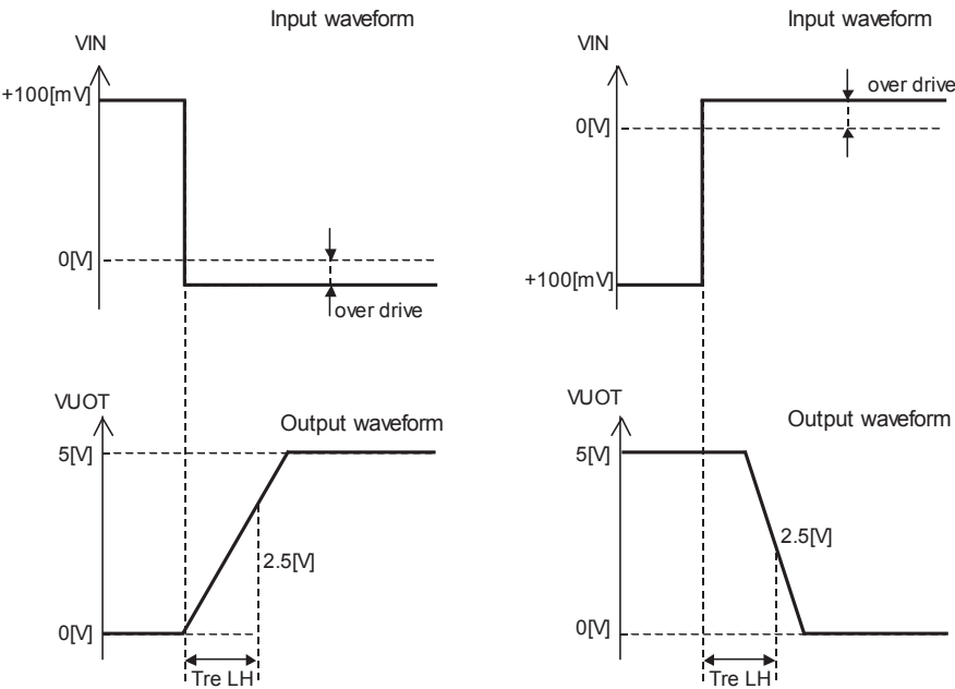
Fig.4 Response Time
