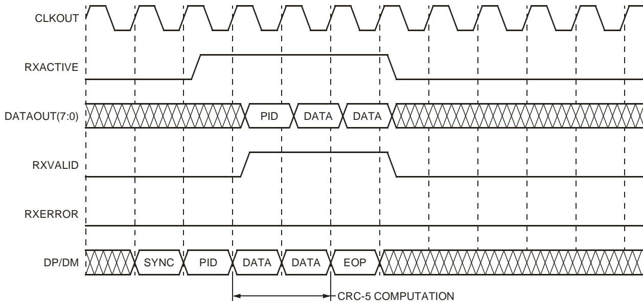
Figure 7. HS Receive Timing for Setup Packet (8-bit)
