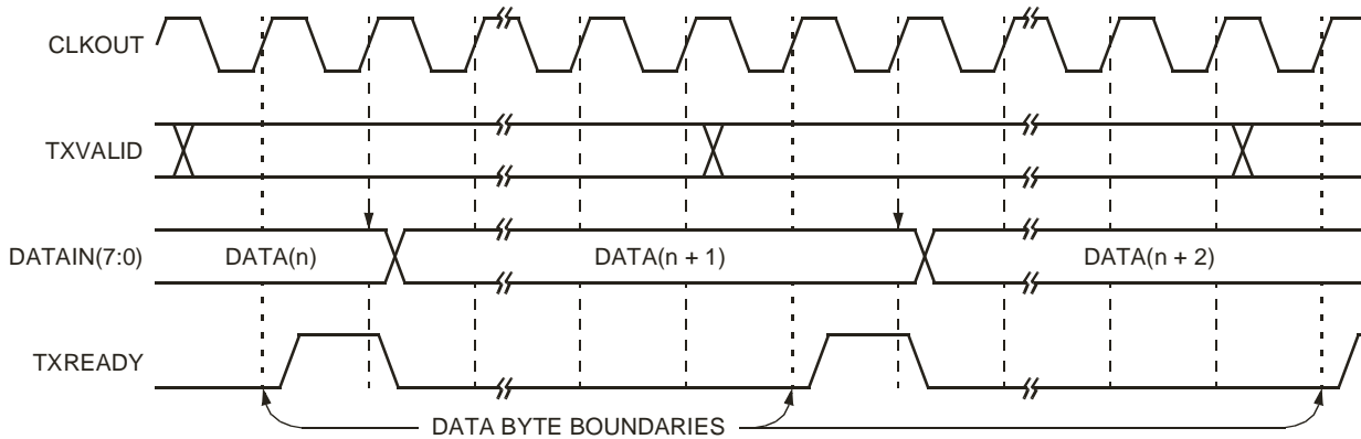
Figure 14. FS CLKOUT Relationship to Transmit Data and Control Signals
