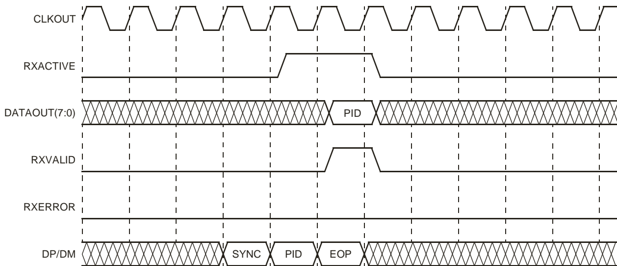
Figure 8. HS Receive Timing for a Handshake Packet (No CRC) (8-bit)
