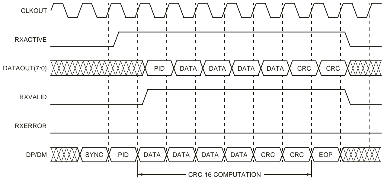
Figure 6. HS Receive Timing for Data Packet (with CRC-16) (8-Bit)
