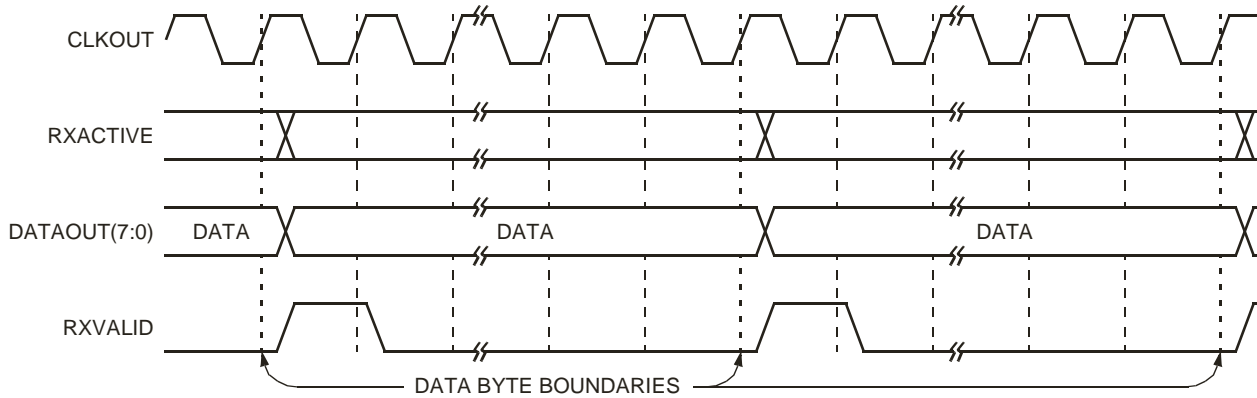
Figure 13. FS CLKOUT Relationship to Receive Data and Control Signals
