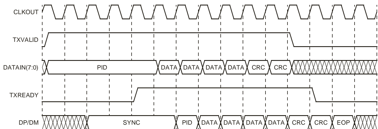
Figure 4. HS Transmit Timing for a Data Packet (8-Bit)
