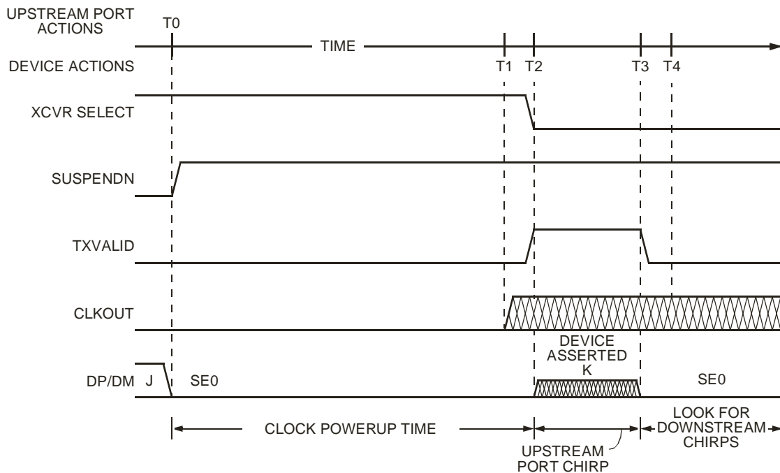
Figure 20. HS Detection Handshake Timing Behavior from Suspend
