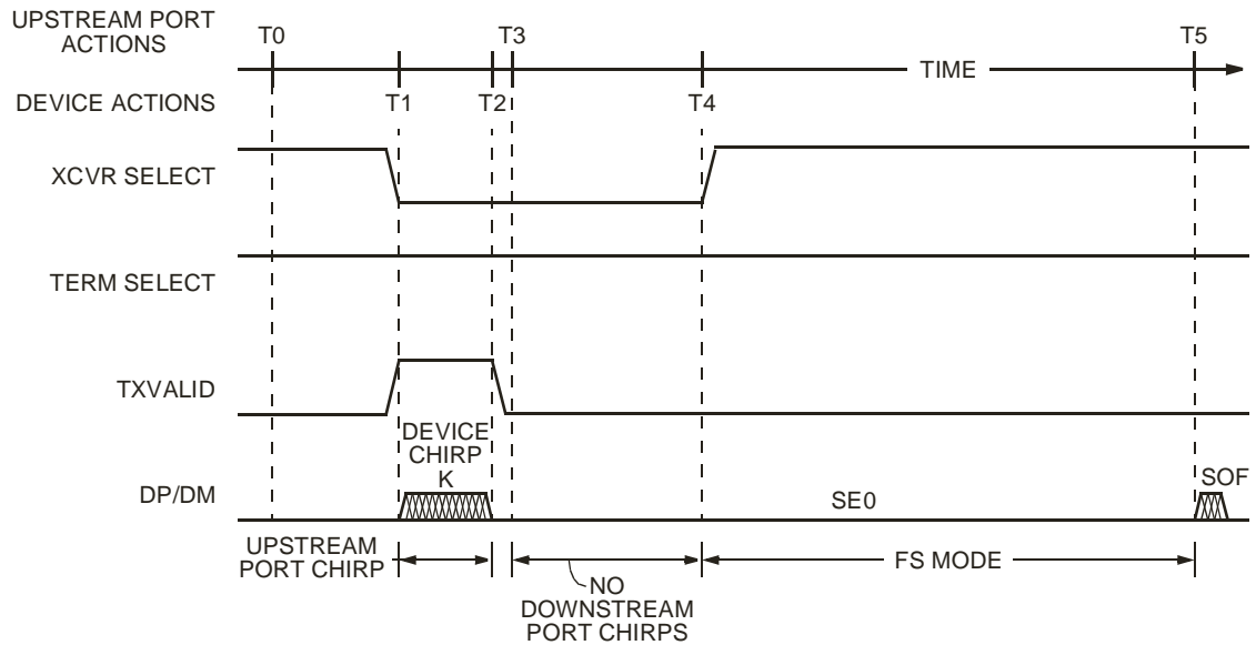
Figure 17. HS Detection Handshake Timing Behavior (FS Mode)
