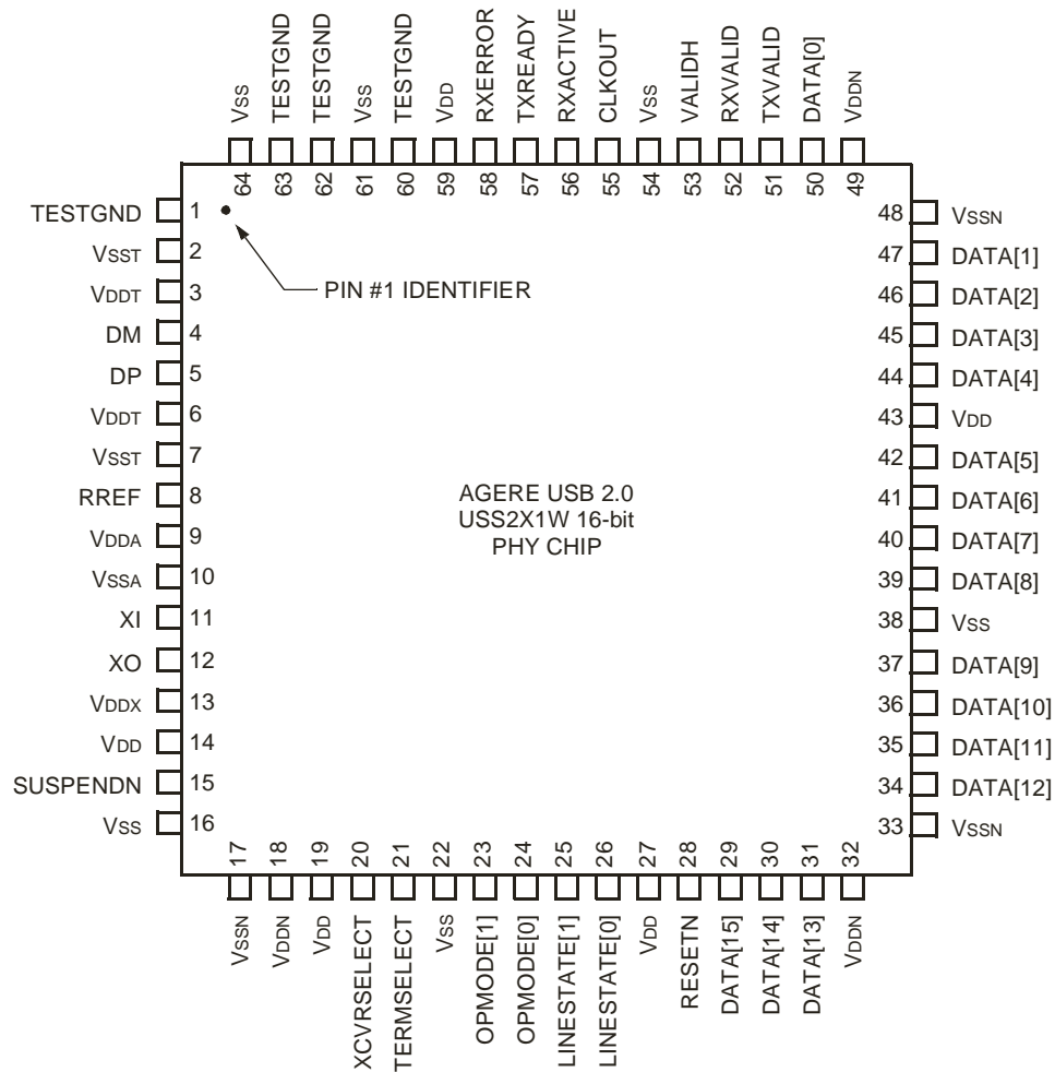
Figure 2. 64-Pin TQFP Package Pin Assignments
