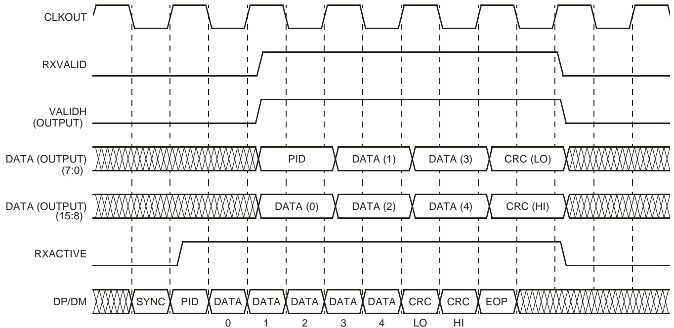
Figure 11. HS Receive Timing for 16-Bit Data, Even Byte Count
