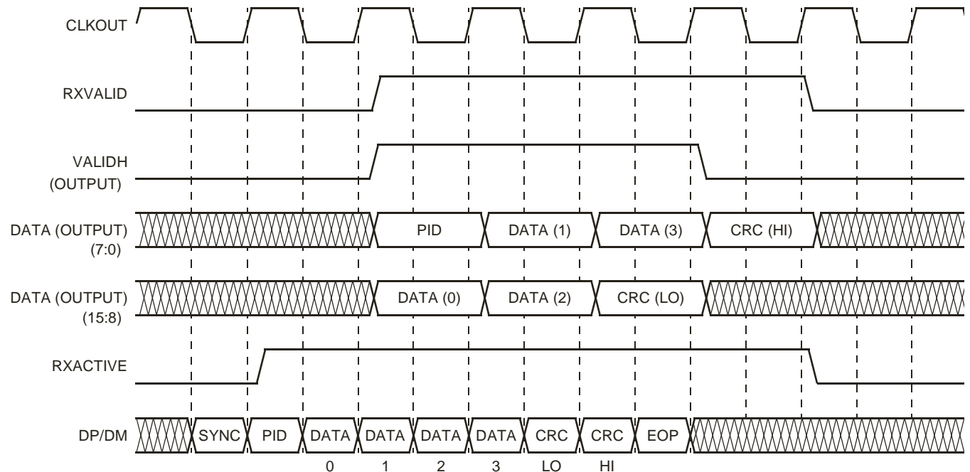
Figure 12. HS Receive Timing for 16-Bit Data, Odd Byte Count
