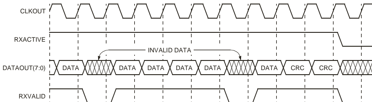
Figure 5. HS Receive Timing for Data with Unstuffing Bits (8-Bit)
