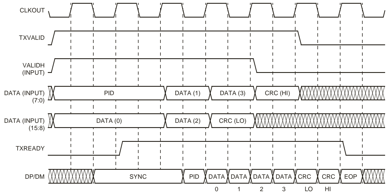
Figure 10. HS Transmit Timing for 16-Bit Data, Odd Byte Count
