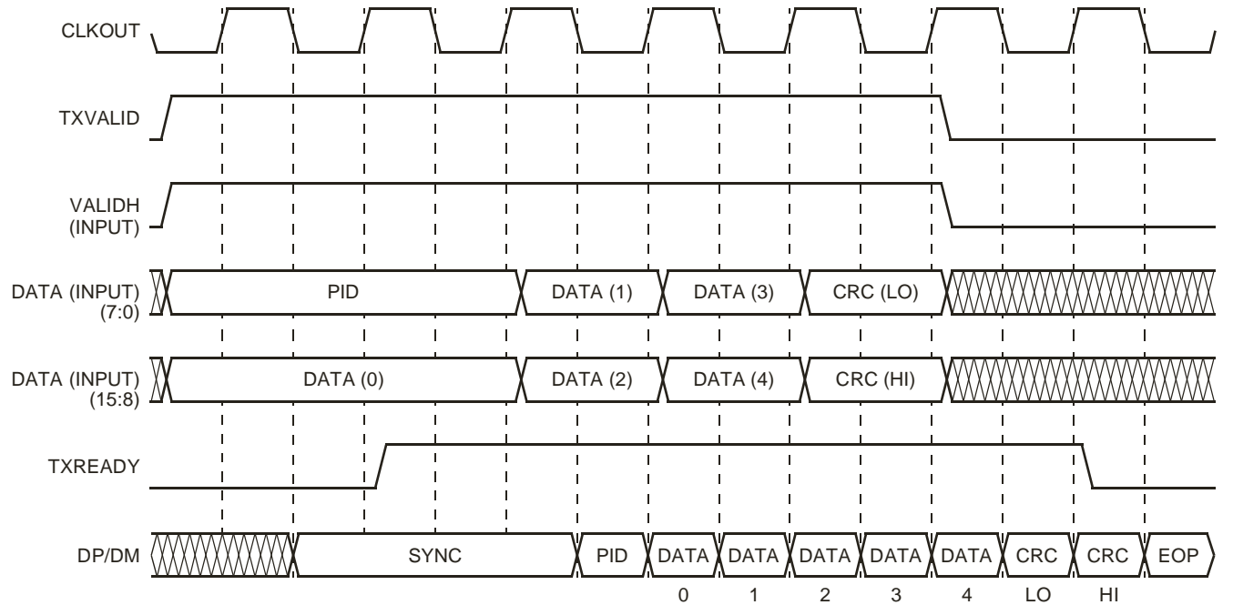
Figure 9. HS Transmit Timing for 16-Bit Data, Even Byte Count
