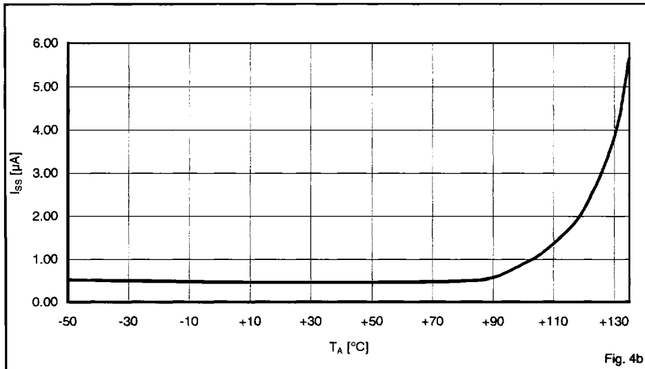
Typical Standby Current at V_{DD} = 5.5\text{ V} and Extended Temperature
