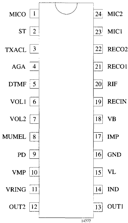
Figure 1. Pinning
