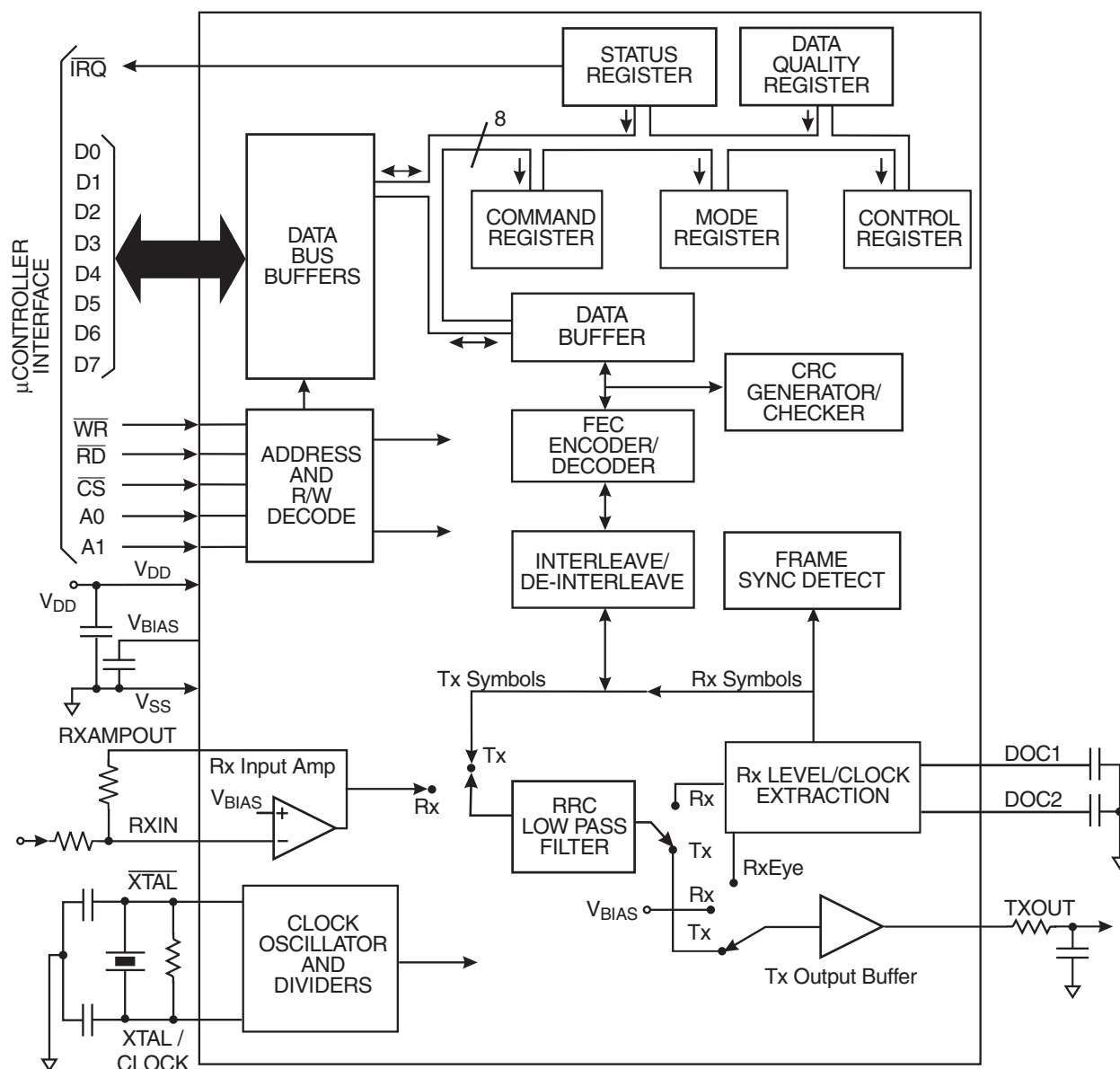
Figure 1: Block Diagram
