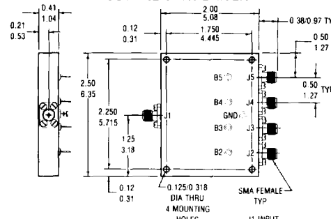
CONFIGURATION R OUTLINE WITHOUT DRIVER
