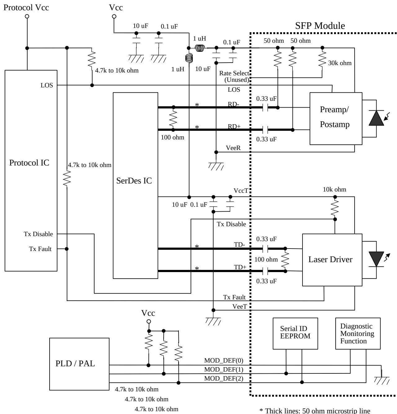
Figure 7. Block Diagram and Recommended Circuit
