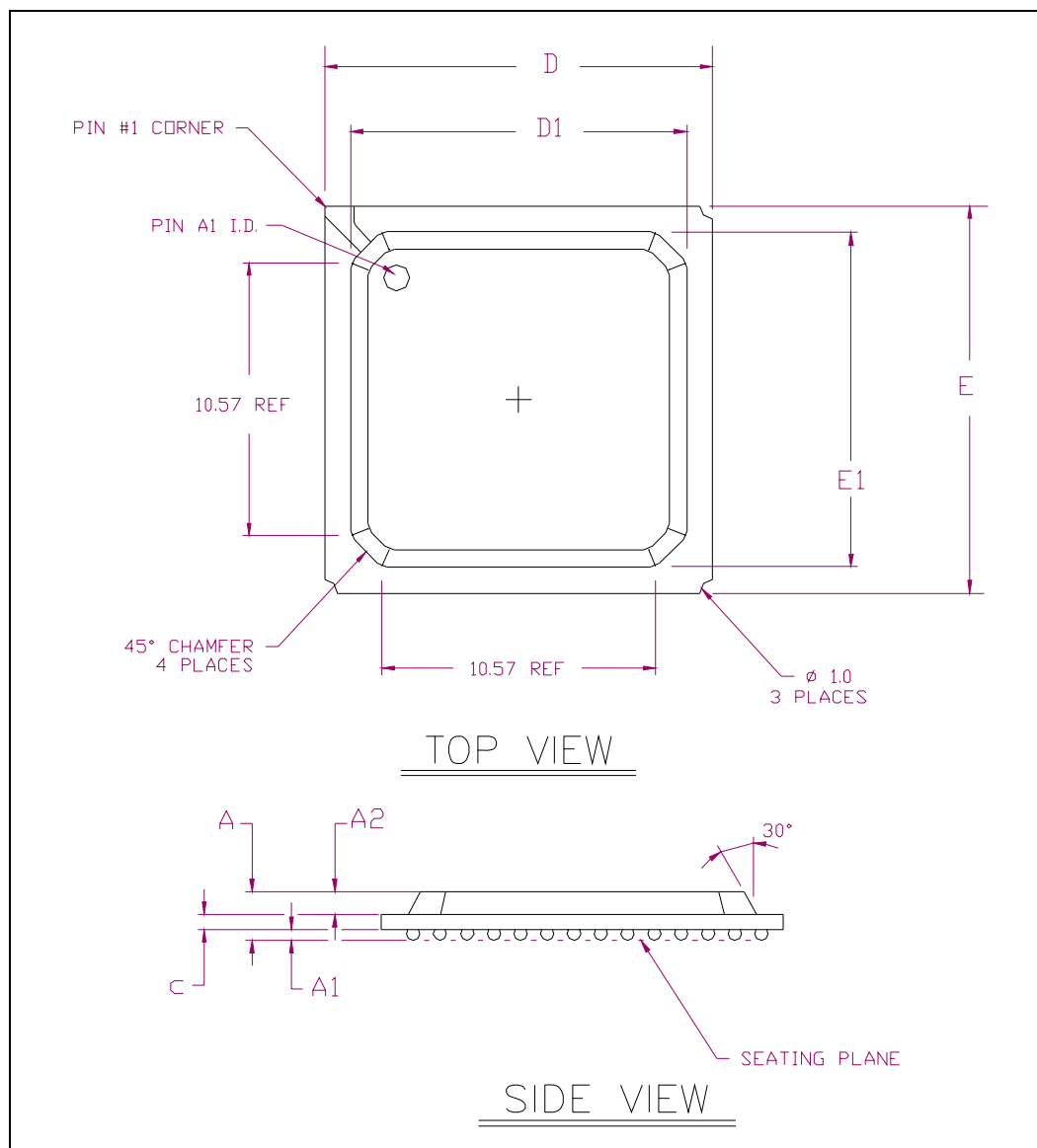
Figure 67. 196-Ball BGA15 Package Specs - Top/Side Views (LXT9785MBC)
