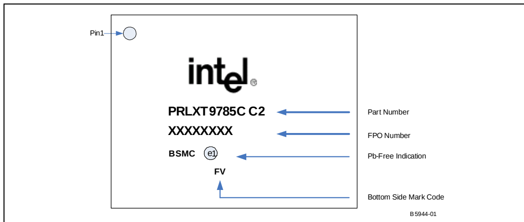
Figure 70. Sample Pb-Free PBGA Package – Intel® LXT9785 Transceiver
