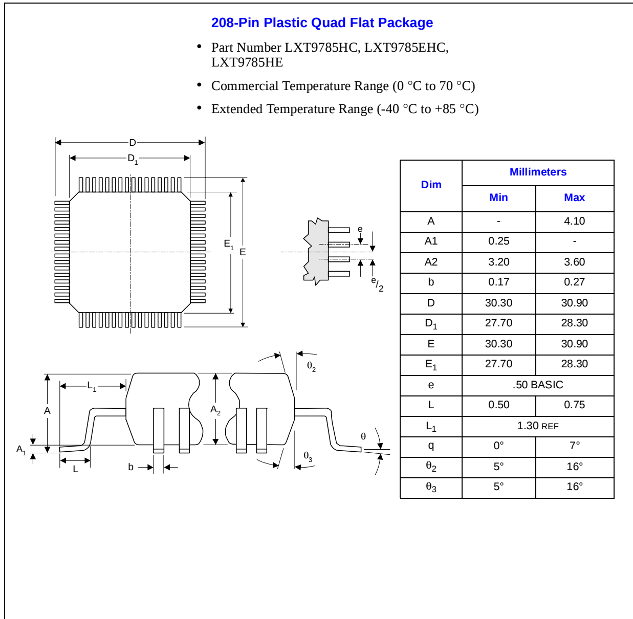
Figure 64. 208-Pin PQFP Plastic Package Specification
