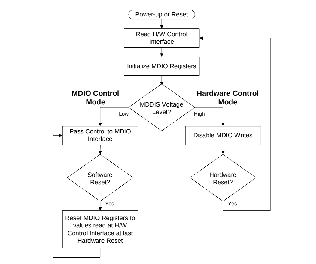
Figure 13. Initialization Sequence
