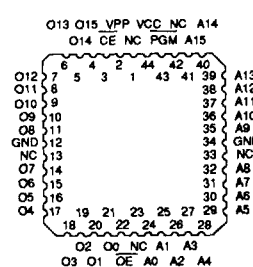
LCC, JLCC, PLCC Top View
