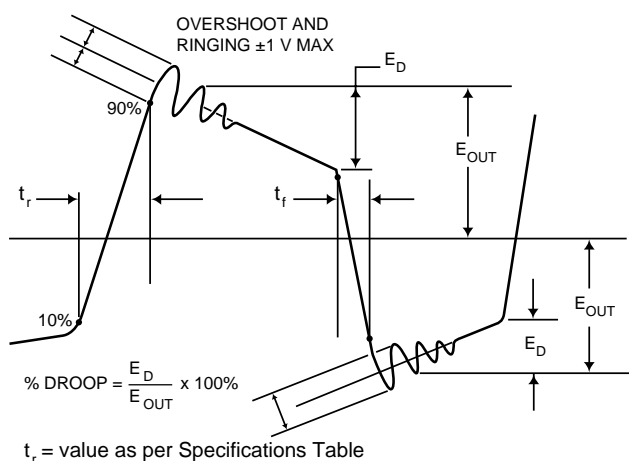
FIGURE 1. WAVEFORM INTEGRITY
