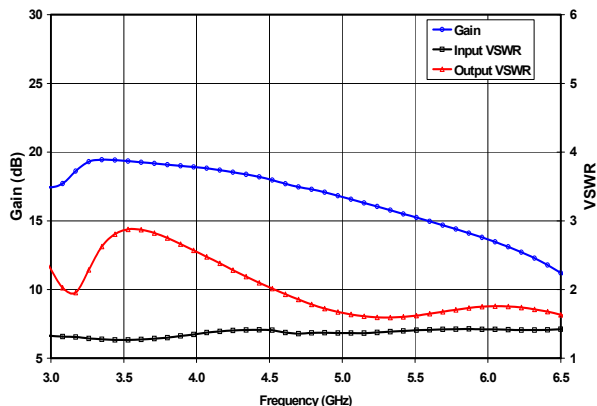
Figure 5. Small Signal Gain and VSWR vs. Frequency at V_{DD} = 8V .
