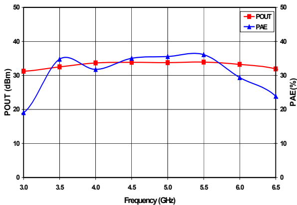
Figure 1. Output Power and Power Added Efficiency vs. Frequency at V_{DD} = 8V and P_{IN} = 20 dBm
