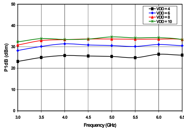
Figure 2. 1dB Compression Point vs. Drain Voltage
