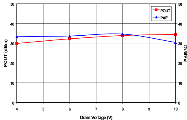
Figure 4. Saturated Output Power and Power Added Efficiency vs. Drain Voltage at f_0 = 4.5 GHz
