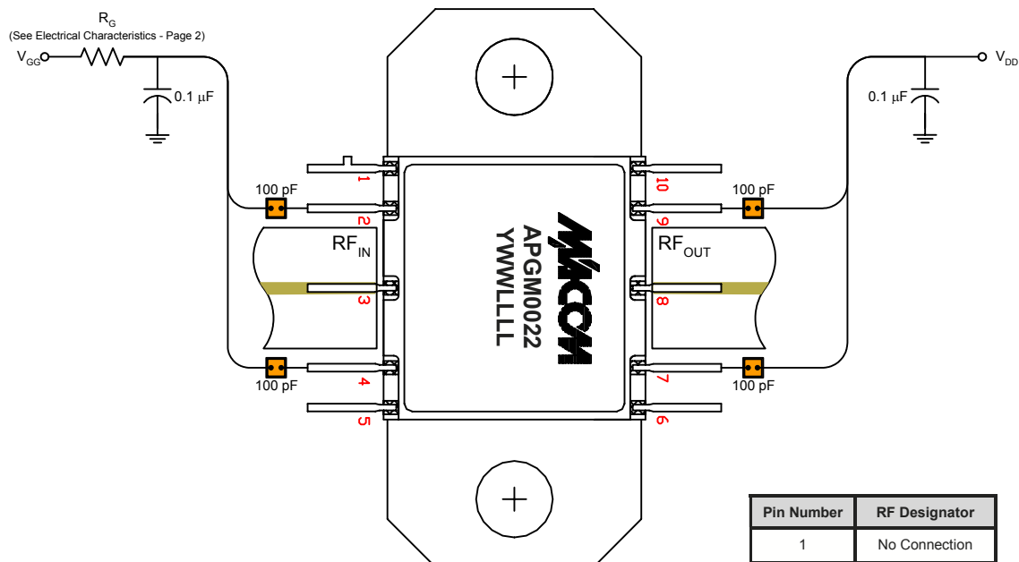
Figure 7. Recommended Bias Configuration
