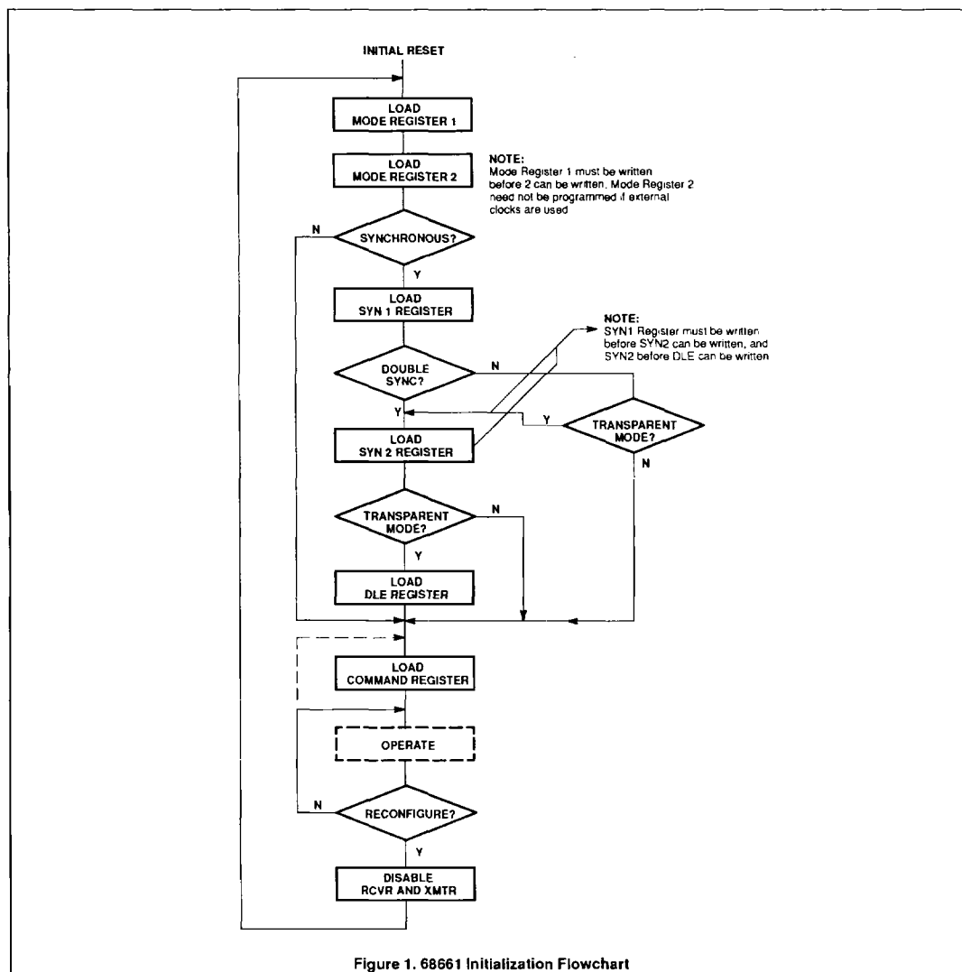
Figure 1. 68661 Initialization Flowchart
