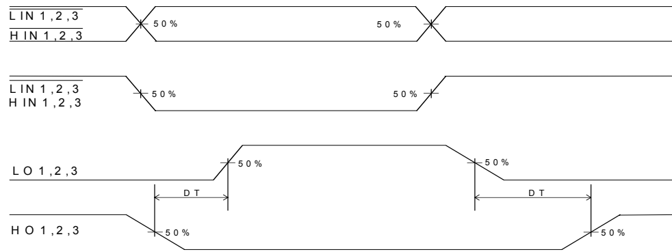
Fig. 4. Internal Deadtime Timing Waveforms
